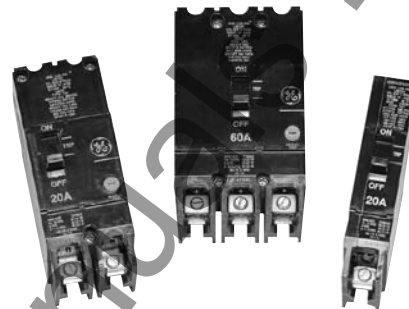
1- 2- and 3-pole TEY breakers
