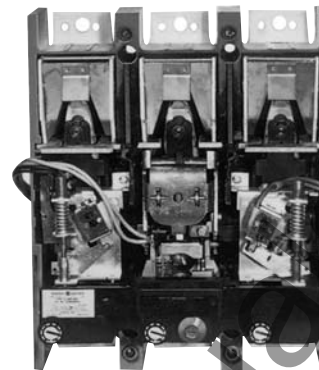
J Frame Circuit Breaker with Internal Accessories Mounted in Each Pole
