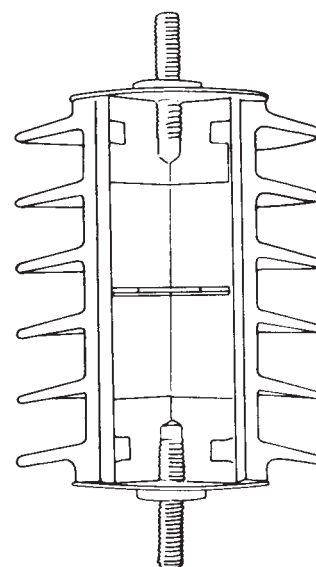
PVR Metal-Oxide Polymer-Housed
