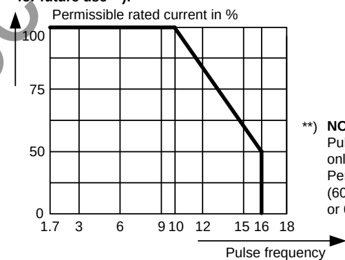
Fig. 11-1 Derating curves
