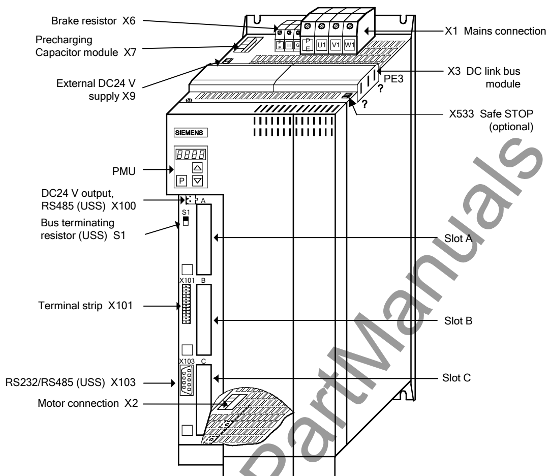
Fig. 7-3 Connection overview for units 180 mm wide
