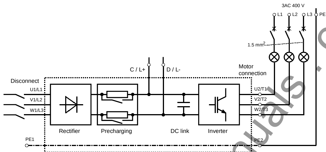
Fig. 10-1 Forming circuit
