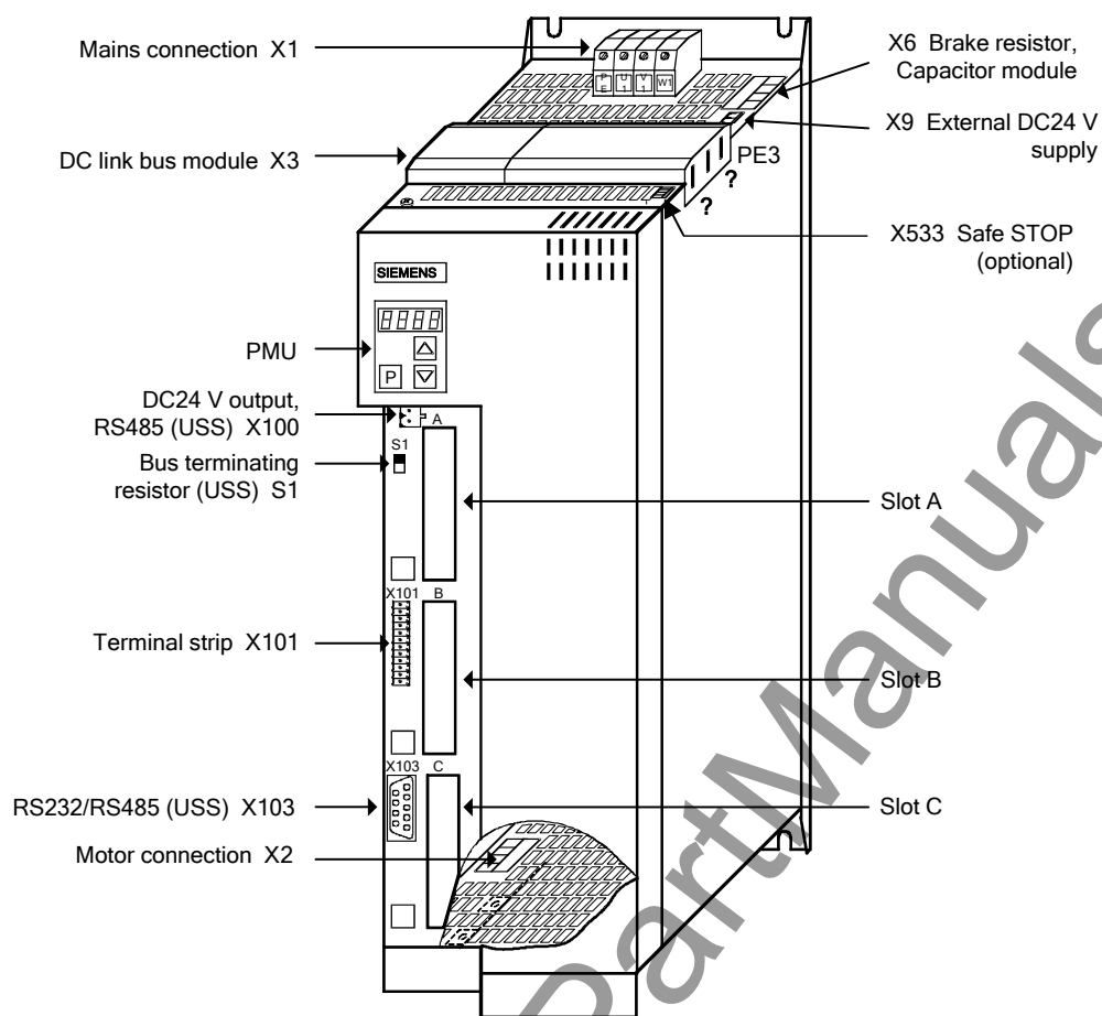
Fig. 7-2 Connection overview for units 135 mm wide
