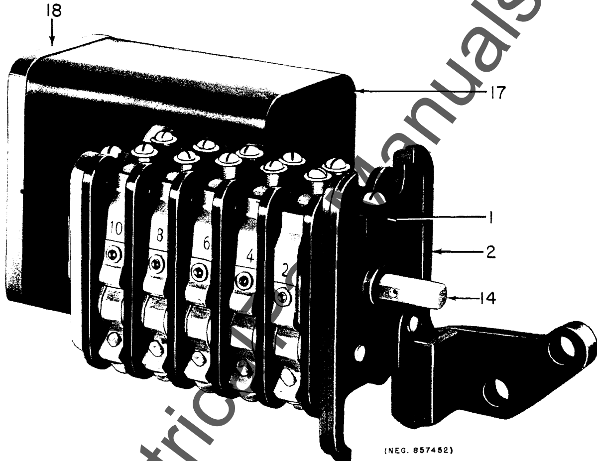
Fig. 1. Typical SB-1 auxiliary switch (cover removed)
