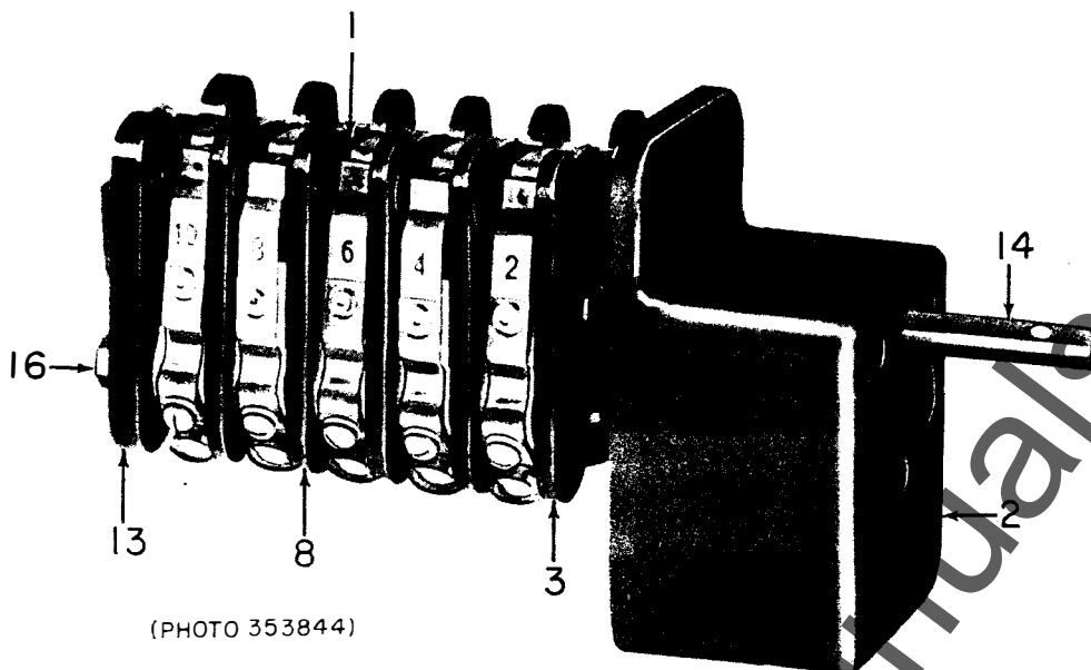
Fig. 2. Typical SB-1 auxiliary switch (cover not shown)
