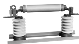
Single-pole fuse holder HF323 with fuse link
