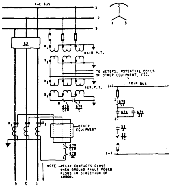
Fig. 5 External Connections of One Type IBC51A Relay Using Auxiliary Wye-Broken-Delta Transformer to Obtain Potential Polarization
