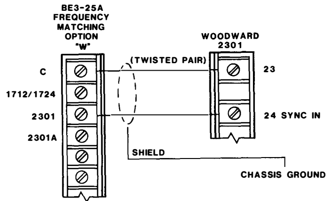
FIGURE 5 – WOODWARD 2301 INTERCONNECTION
