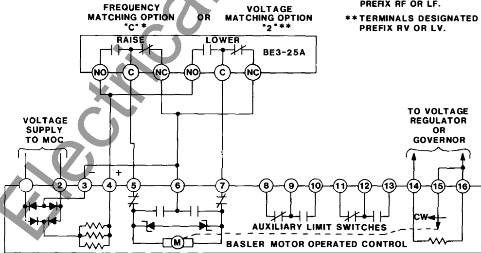
FIGURE 8 – RAISE/LOWER CONTACT INTERCONNECTION
