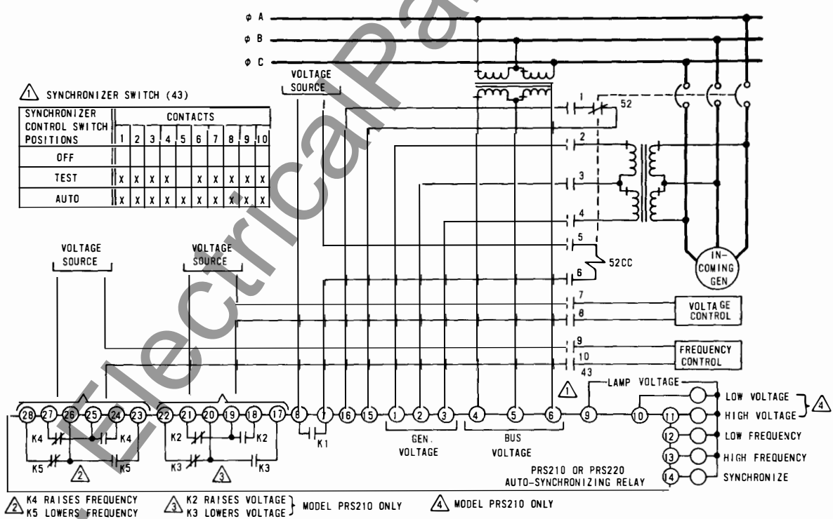
FIGURE 4: TYPICAL INTERCONNECTION
