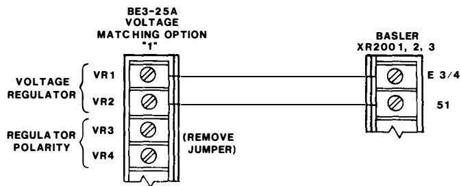
FIGURE 9 – BASLER XR2001, XR2002, XR 2003 INTERCONNECTION
