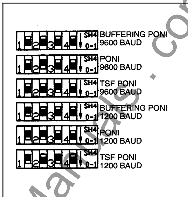
Fig. 10 Function Selection Switch
