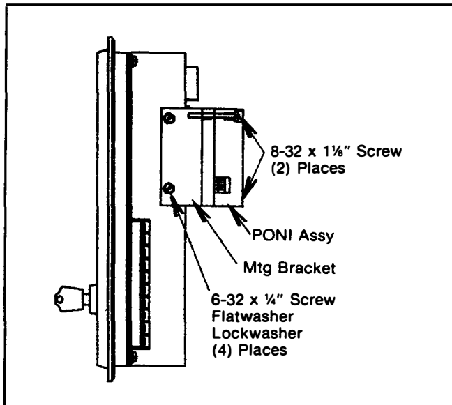
Fig. 4 IQ 1000 Mounting
