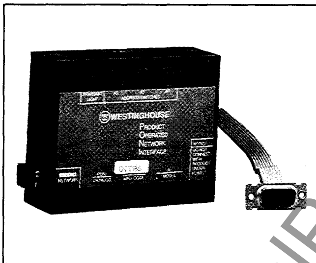
Fig. 1 The Westinghouse PONI
