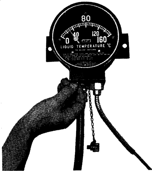
FIG. 3. Method of Resetting Maximum Indicating Pointer. Maximum Pointer Shown Reset.
