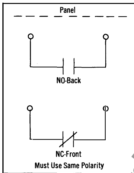
Figure 3 - Internal Wiring Diagrams
