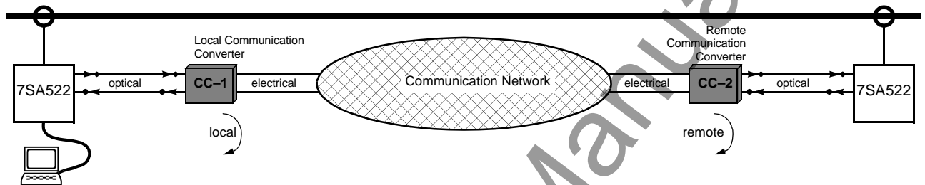
Figure 8-21 Distance protection communication via communication converter and communication network - example
