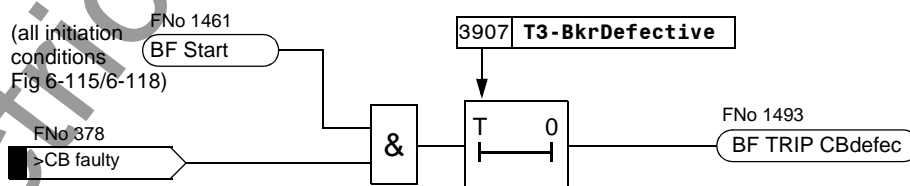
Figure 6-122 Circuit breaker not operational
