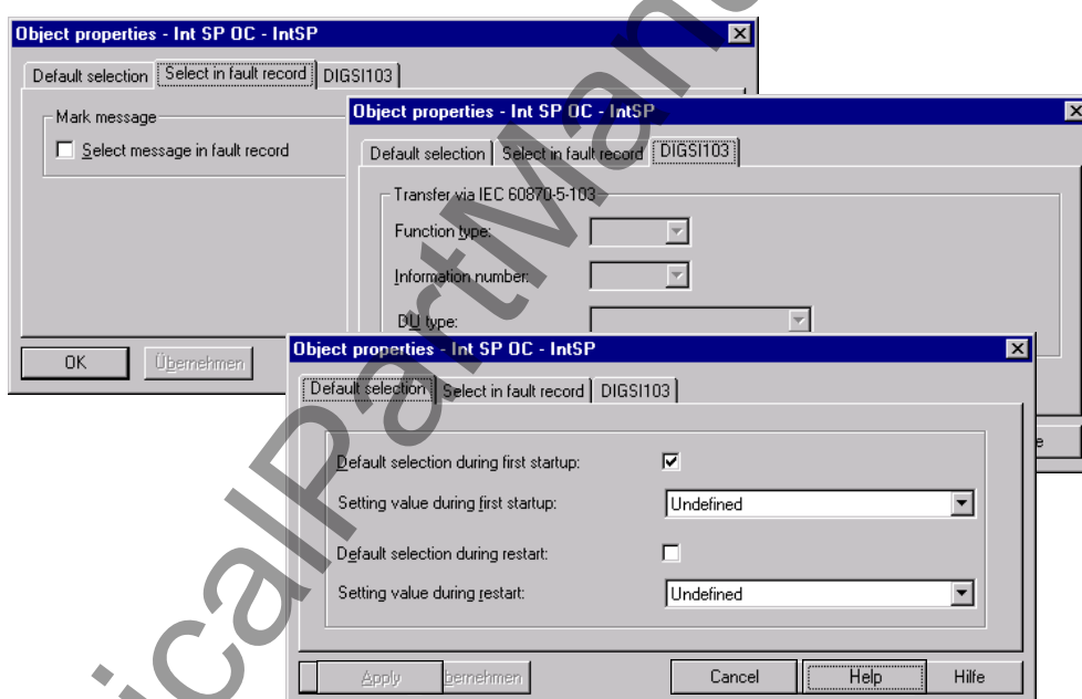
Figure 5-12 Information properties — example for the information type “Internal Single Point Indication” (IntSP)
