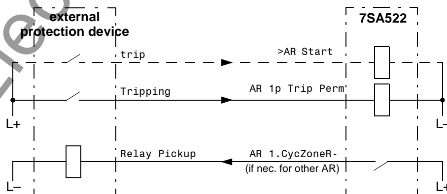
Figure 6-99 Connection example with external protection device for 3-pole reclosure; AR control mode = with TRIP
