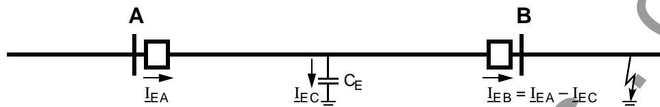
Figure 6-82 Possible current distribution during external earth fault
