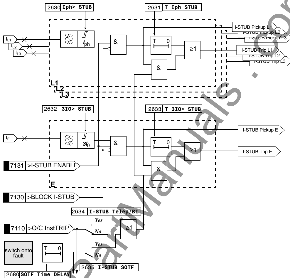
Figure 6-89 Logic diagram of the stub protection
