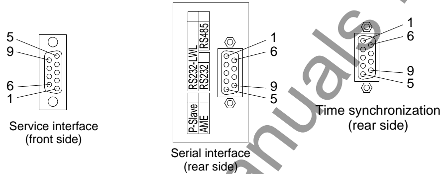
Figure 2-16 9 pin D-subminiature connector
