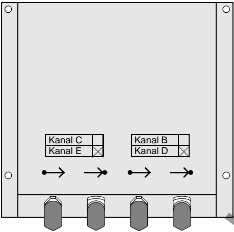
Figure 2-22 Inclined housing with fibre-optic connections (channel D and E fitted)
