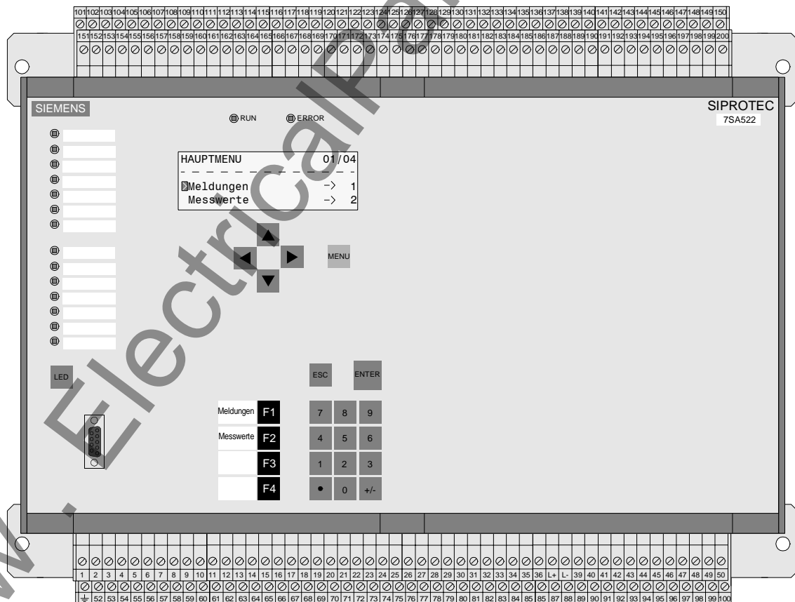
Figure 2-18 Front view of a 7SA522, housing size 1 / 1 , for panel surface mounting, without optical connections
