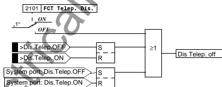
Figure 6-52 Switching on and off of the teleprotection
