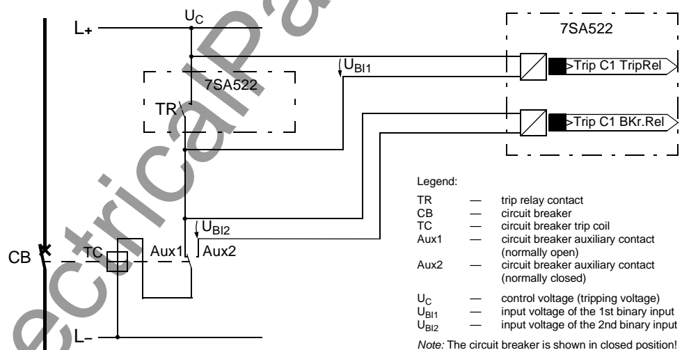
Figure 6-133 Trip circuit supervision operating principle with two binary inputs
