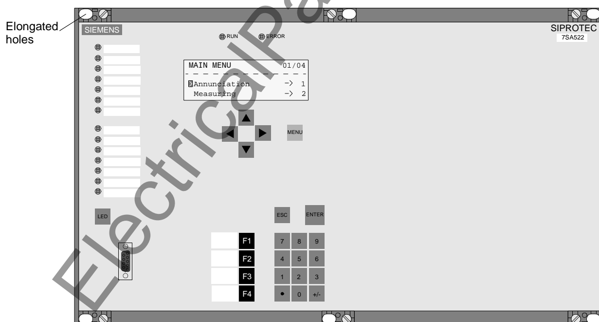
Figure 8-2 Panel mounting of a 7SA522 (housing width \frac{1}{4} of 19 inch rack)
