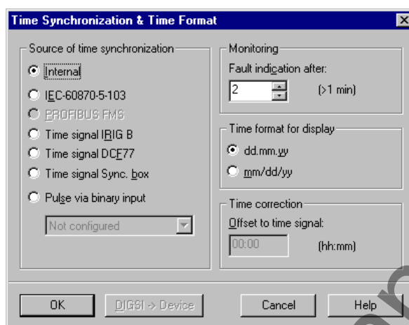
Figure 5-48 Dialogue box for time synchronization and format in DIGSI® 4 – example
