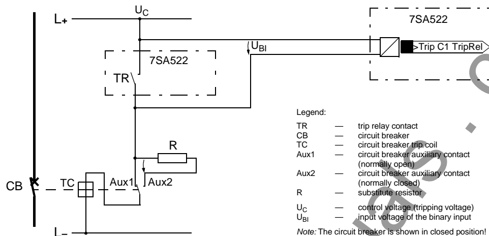
Figure 6-135 Operating principle of the trip circuit supervision with one binary input
