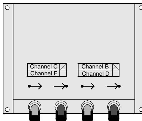
Figure 2-20 Inclined housing with fibre optic connections (example: channel B and C fitted)
