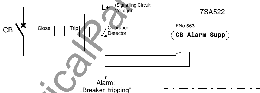
Figure 6-143 Breaker Tripping Alarm Suppression
