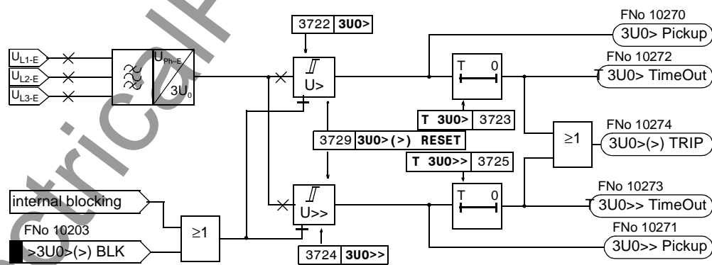
Figure 6-106 Logic diagram of the overvoltage protection for zero sequence voltage
