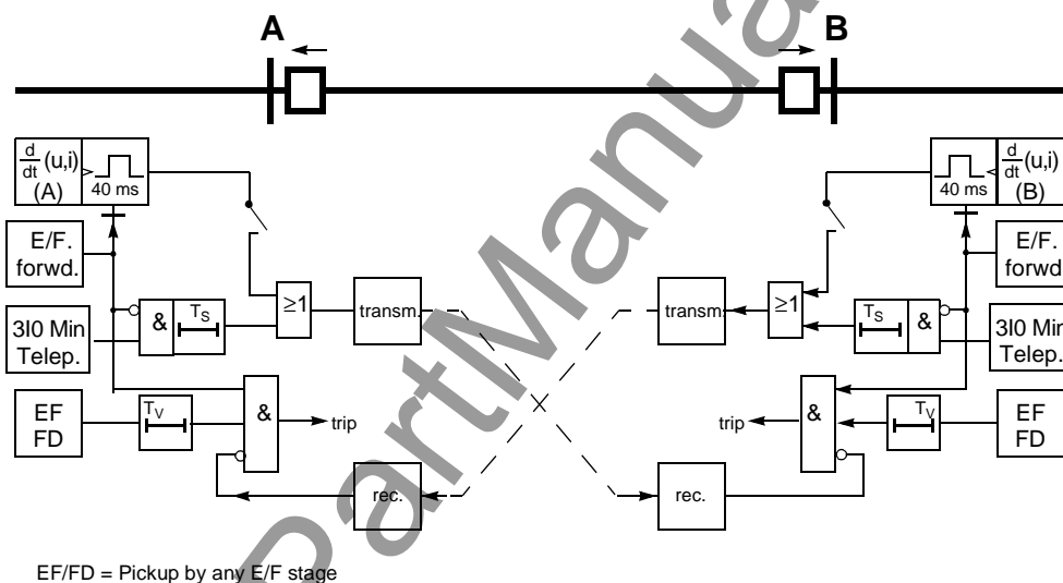
Figure 6-78 Operation scheme of the directional blocking method
