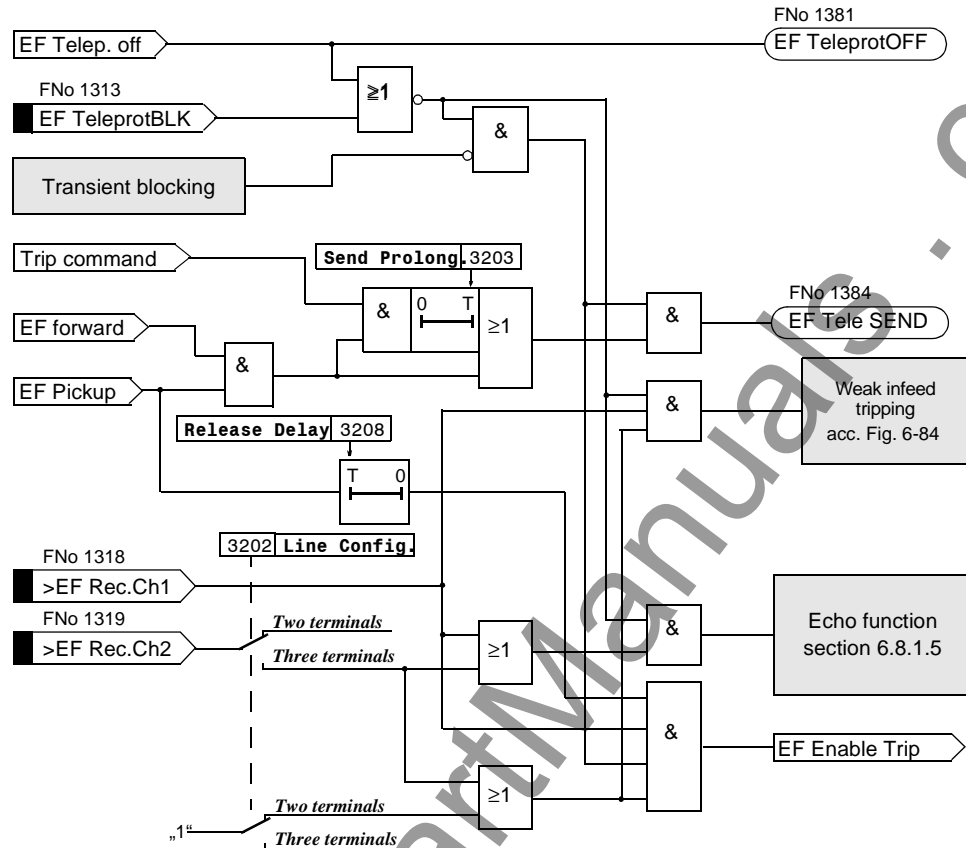
Figure 6-74 Logic diagram of the directional comparison scheme (one line end)
