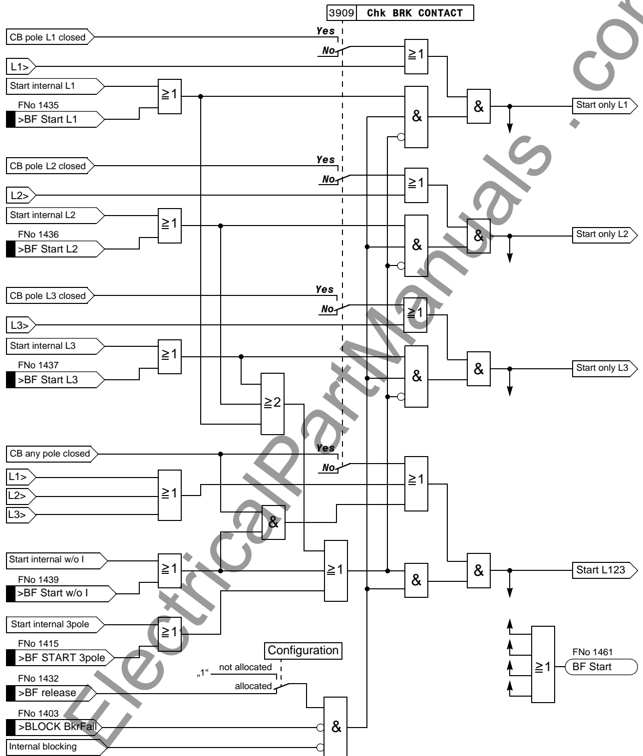
Figure 6-118 Initiation conditions with phase segregated initiation
