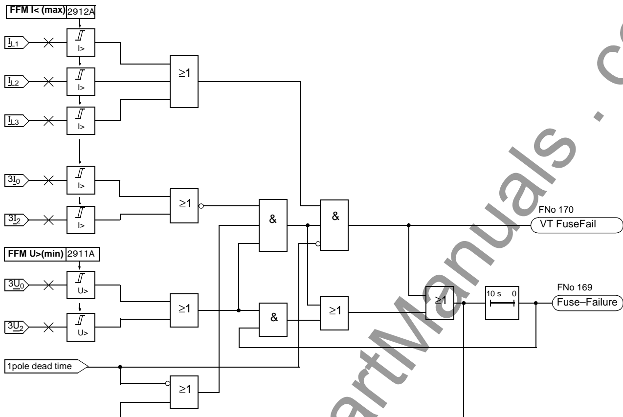
Figure 6-131 Logic diagram of the fuse failure monitor with zero and negative sequence system
