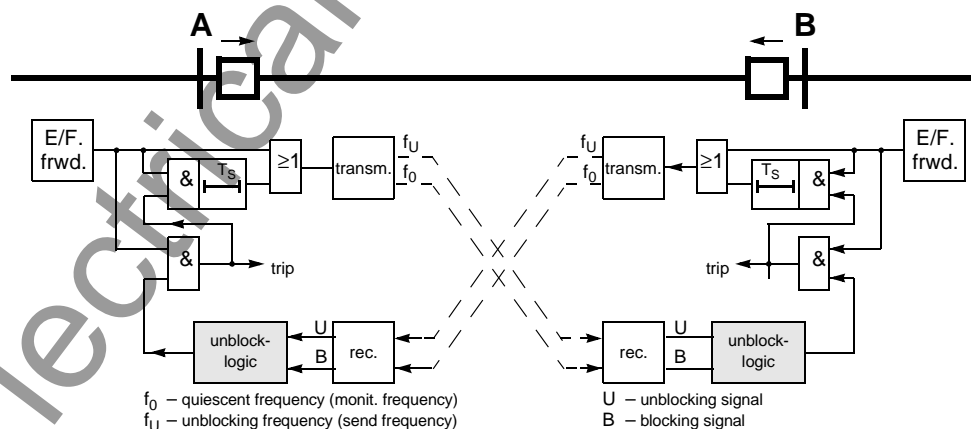
Figure 6-76 Operation scheme of the directional unblocking method
