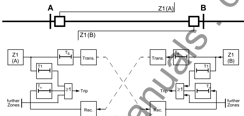
Figure 6-55 Operation scheme of the direct underreach transfer trip method
