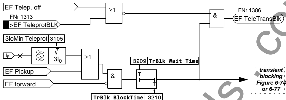
Figure 6-80 Transient blocking for a directional comparison and directional unblocking schemes
