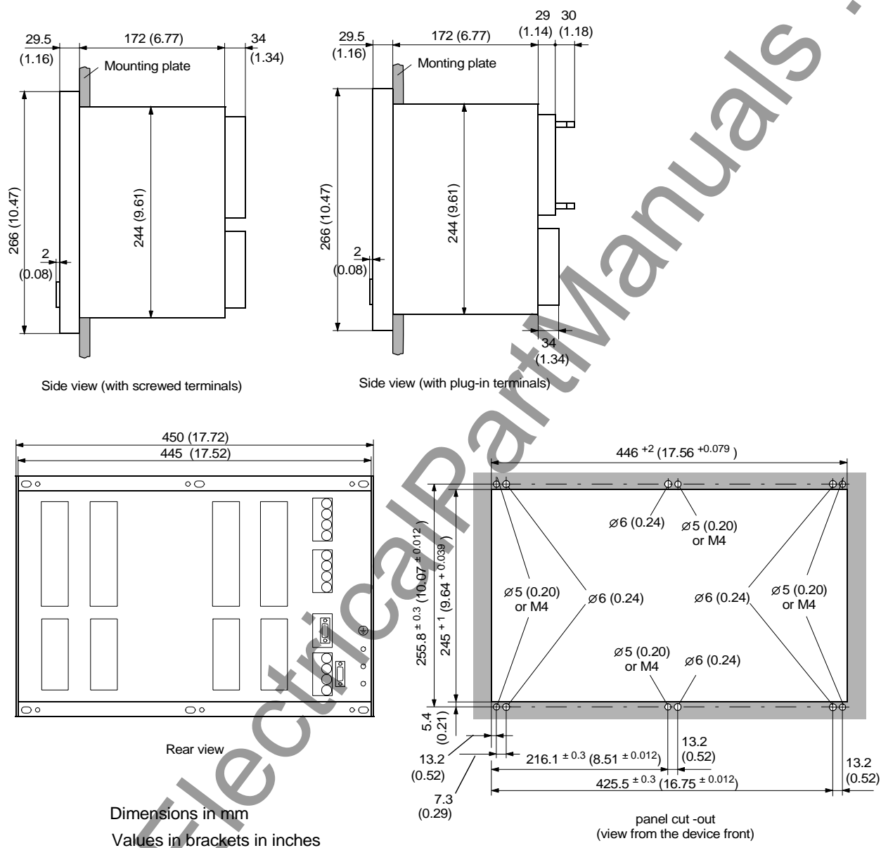
Figure 10-6 Dimensions 7SA522 for panel flush mounting or cubicle installation (size 1\frac{1}{4} x 19")
