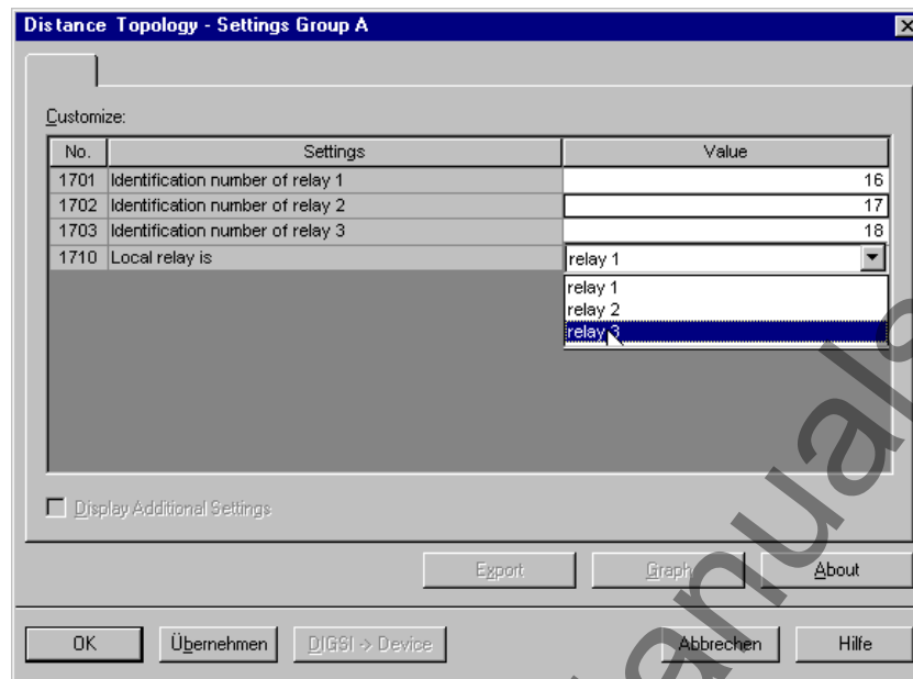
Figure 6-51 Distance Protection topology for 3 ends with 3 devices - example
