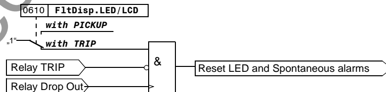
Figure 6-145 Logic diagram of the trip dependent messages
