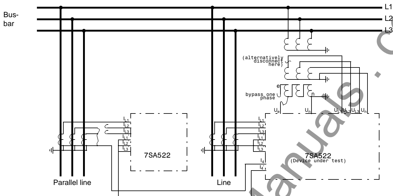
Figure 8-25 Polarity check of I_4 , example with earth current of a parallel line
