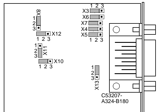
Figure 8-13 Location of the jumpers for configuration of RS232
