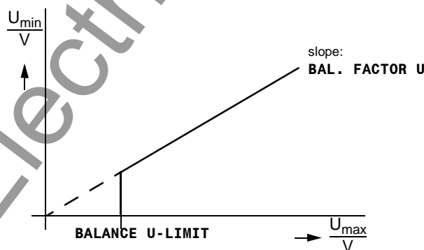
Figure 6-130 Voltage symmetry monitoring
