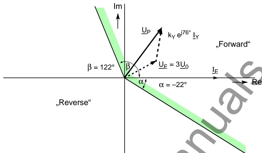
Figure 6-70 Directional characteristic of the earth fault protection
