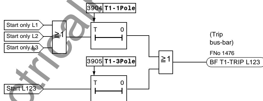
Figure 6-120 Single-stage breaker failure protection with different delay timers
