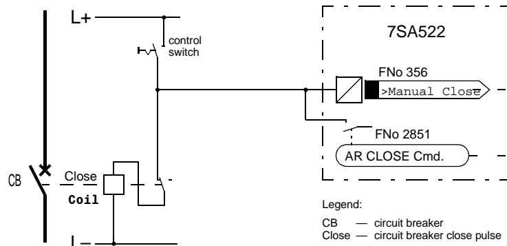
Figure 6-138 Manual closure with internal automatic reclosure
