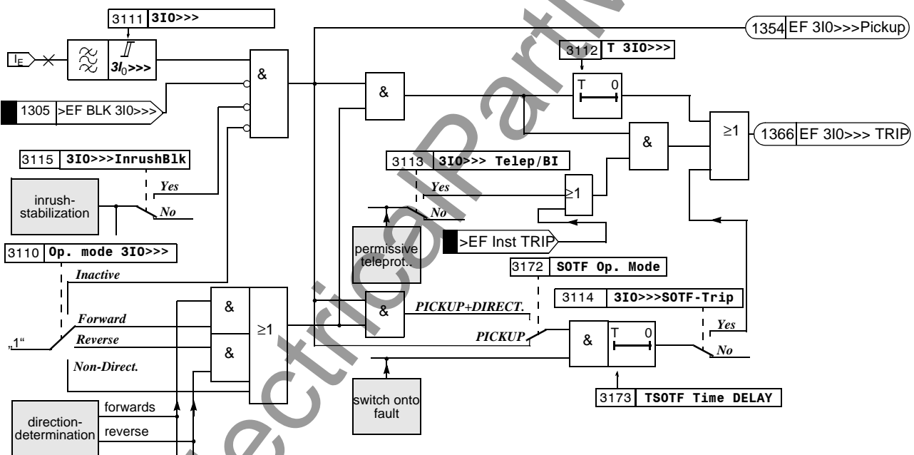
Figure 6-66 Logic diagram of the 3I_0>>> -stage
