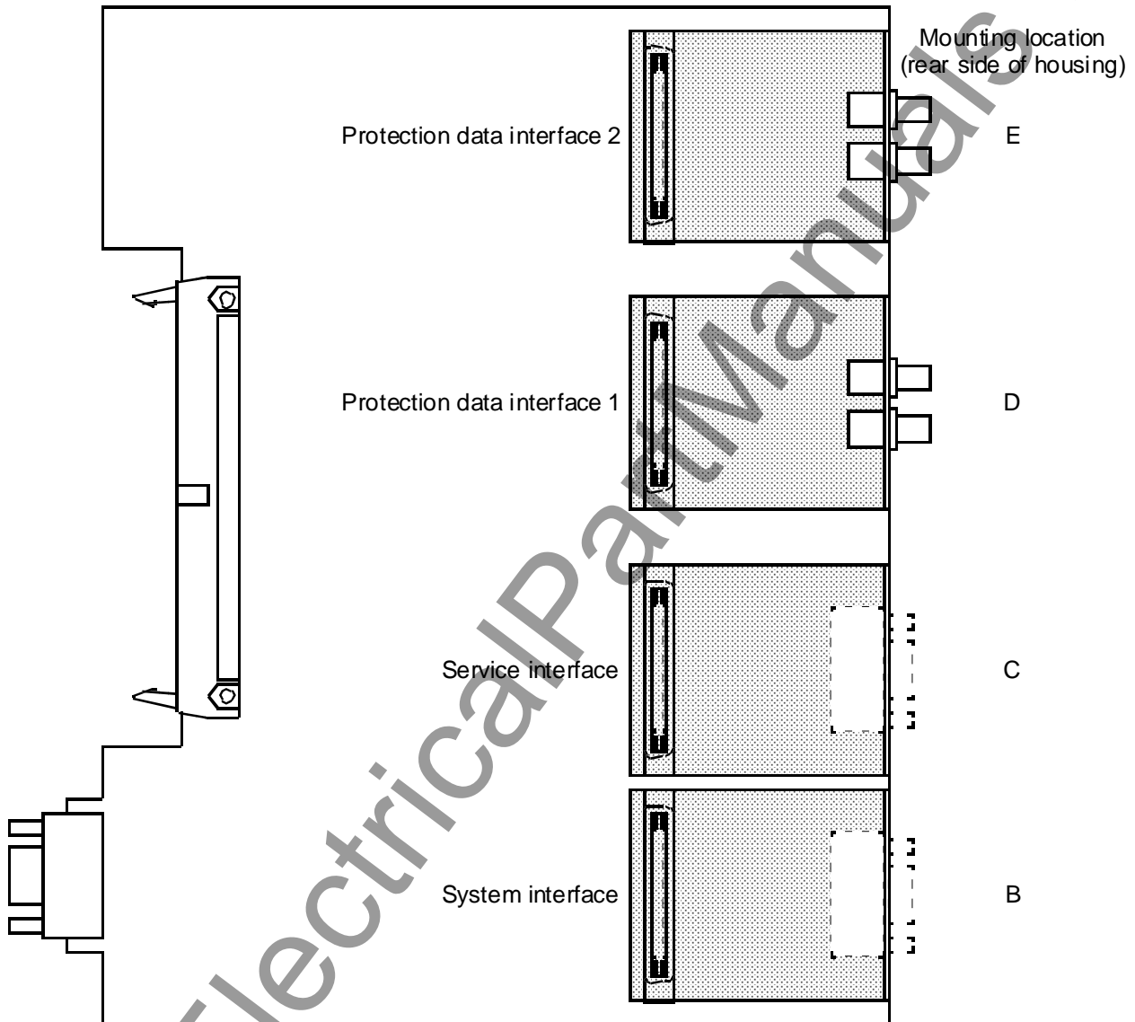
Figure 8-12 Processor board C-CPU-1 and the interface modules (max. complement)
