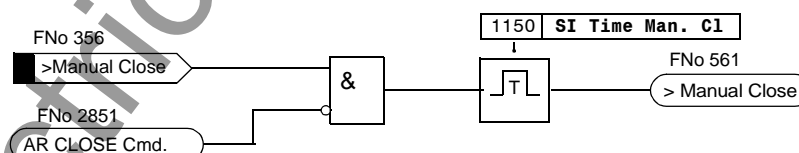
Figure 6-137 Logic diagram of the manual closure handling
