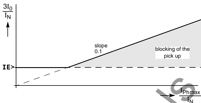
Figure 6-69 Phase current stabilization
