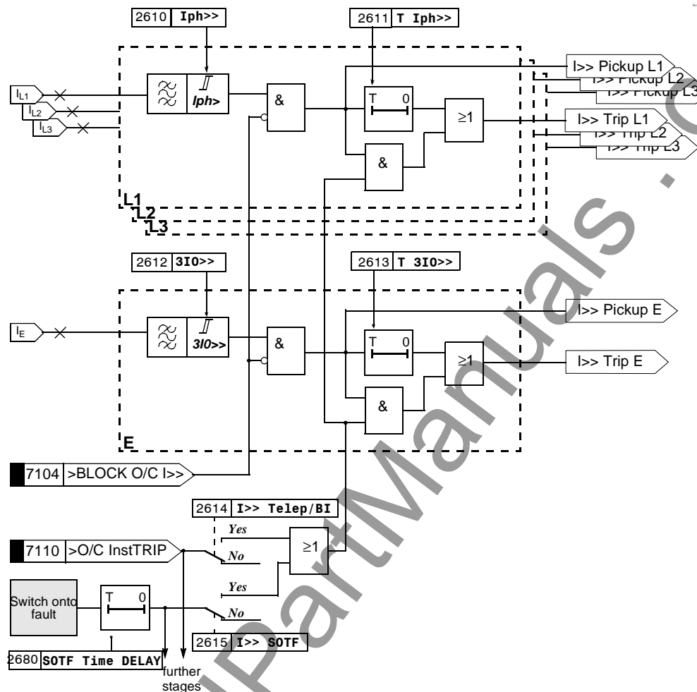
Figure 6-86 Logic diagram of the I&gt;&gt;-stage
