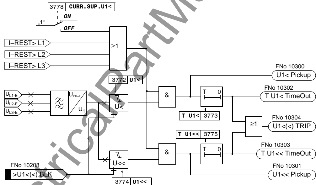
Figure 6-108 Logic diagram of the undervoltage protection for positive sequence voltage system
