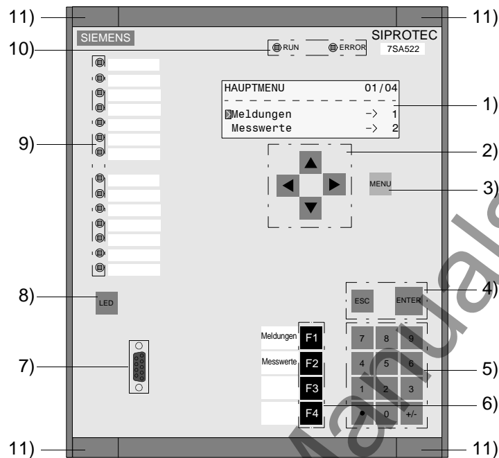
Figure 2-1 Front view of a 7SA522, housing size 1\frac{1}{2} , for panel flush mounting or cubicle mounting
