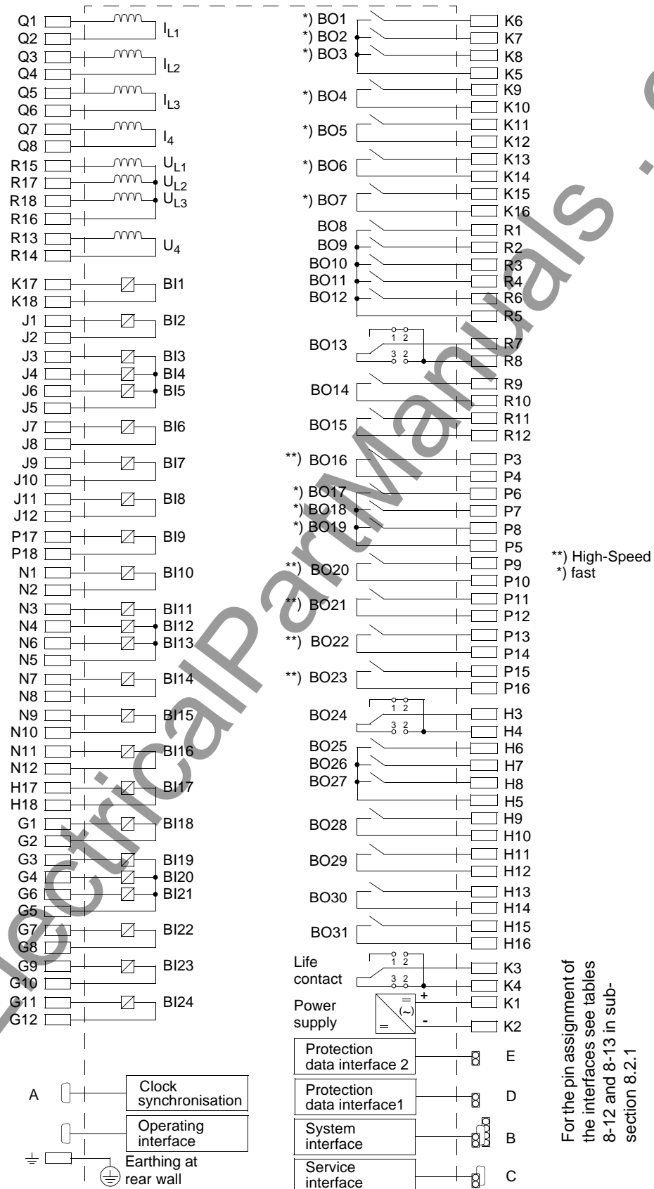
Figure A-5 General diagram 7SA522*-*P/T (panel flush mounting or cubicle mounting; size 1 /1)
