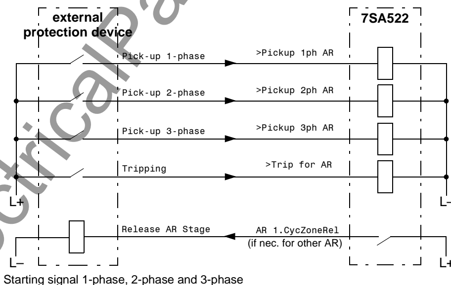
Figure 6-100 Connection example with external protection device for fault detection dependent dead time — dead time control by start signals of the protection device; AR control mode = with PICKUP
