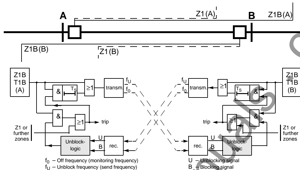
Figure 6-58 Operation scheme of the unblocking method with Z1B
