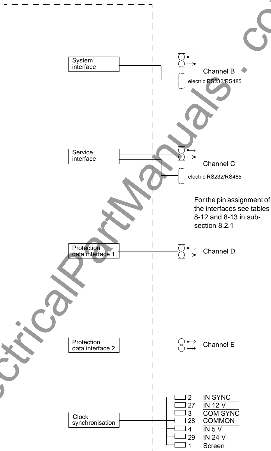
Figure A-8 General diagram 7SA522*—*E beginning with development state /EE (panel surface mounting; size 1\frac{1}{2} )
