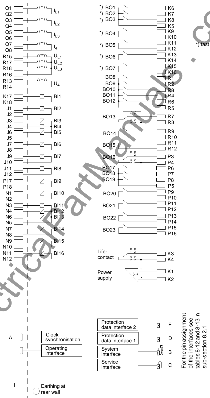
Figure A-2 General diagram 7SA522*-*C/L (panel flush mounting or cubicle mounting; size 1 / 1 )
