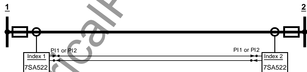
Figure 6-46 Distance protection for two ends with two 7SA522 devices, each of them having one protection data interface (transmitter/ receiver)
