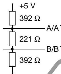
Figure 8-16 Termination of interface RS485 (external)
