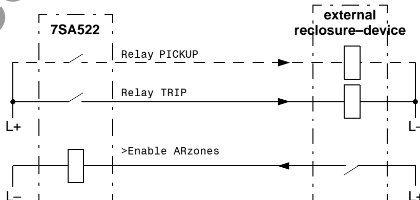
Figure 6-97 Connection example with external reclosure device for 3-pole reclosure
