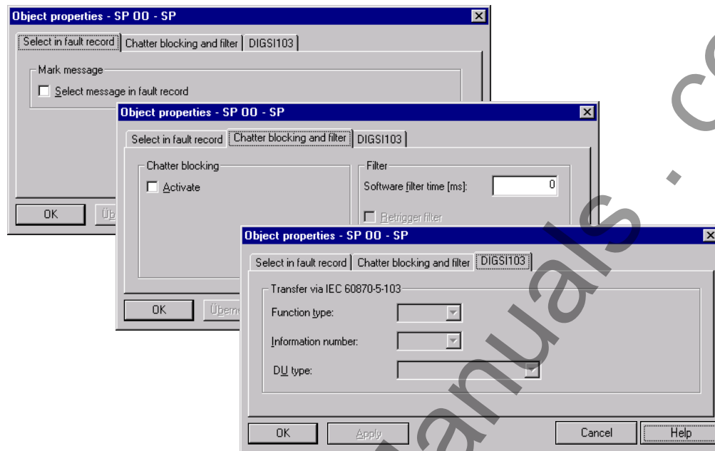
Figure 5-13 Information properties — example for information type “Single Point Indication” (SP)
