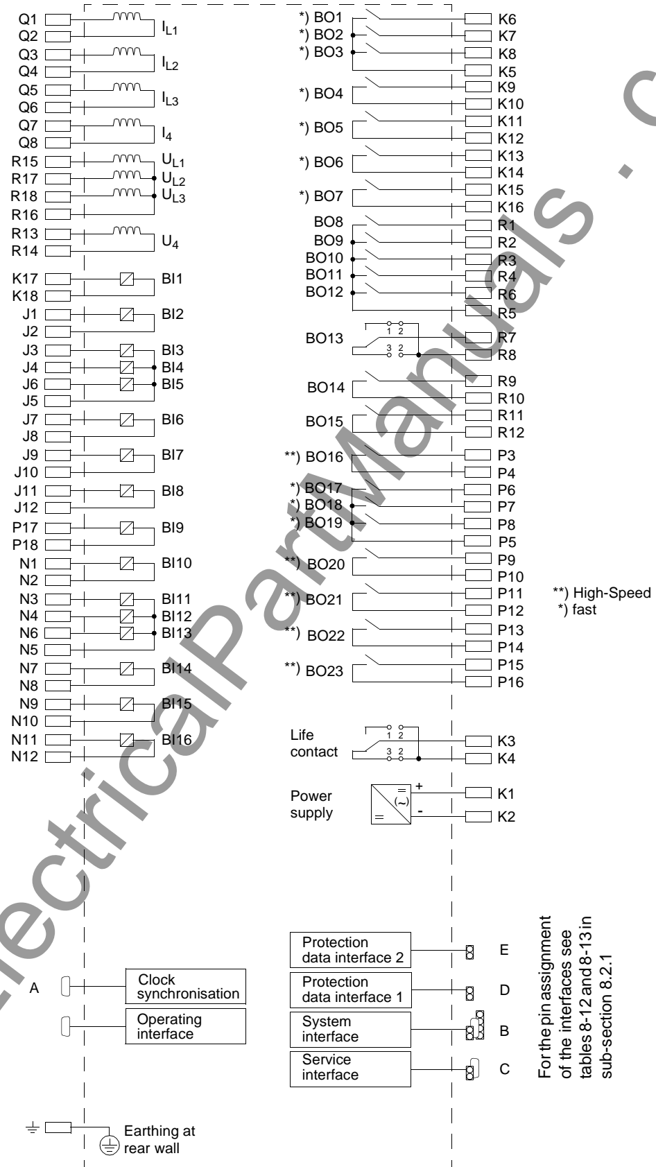
Figure A-3 General diagram 7SA522*-*N/S (panel flush mounting or cubicle mounting; size 1 / 1 )
