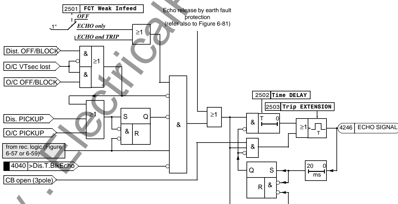
Figure 6-64 Logic diagram of the echo function with distance protection teleprotection
