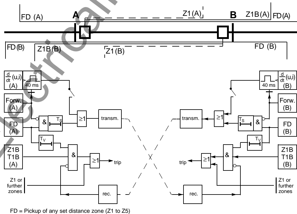
Figure 6-61 Operation scheme of the blocking method
