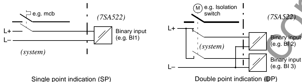
Figure 5-3 Input indications
