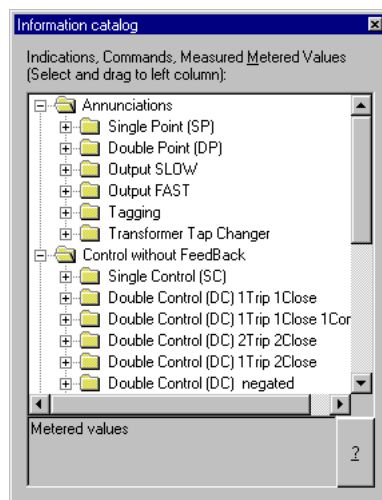
Figure 5-21 Information catalog window — example
