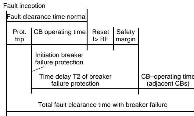
Figure 6-127 Time sequence example for normal clearance of a fault, and with circuit breaker failure, using single-stage breaker failure protection
