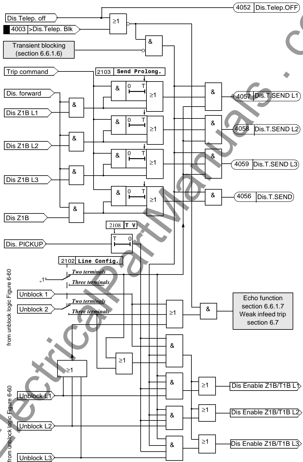
Figure 6-59 Logic diagram of the unblock scheme with Z1B (one line end)
