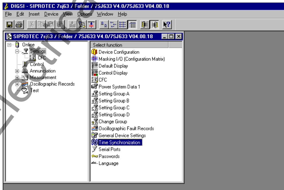
Figure 5-47 Setting Window in DIGSI® 4 – example
