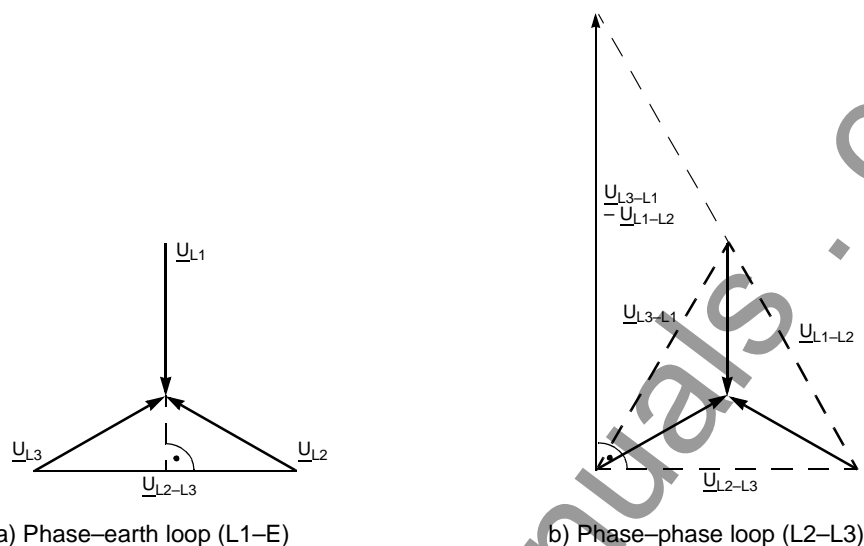
Figure 6-26 Direction determination with quadrature voltages
