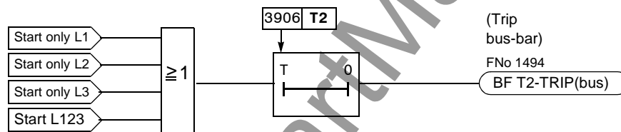
Figure 6-119 Single-stage breaker failure protection with common phase initiation
