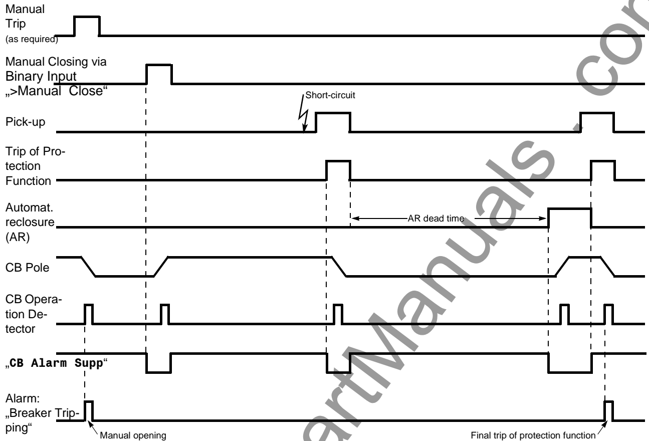
Figure 6-144 Breaker Tripping Alarm Suppression — Sequence Examples
