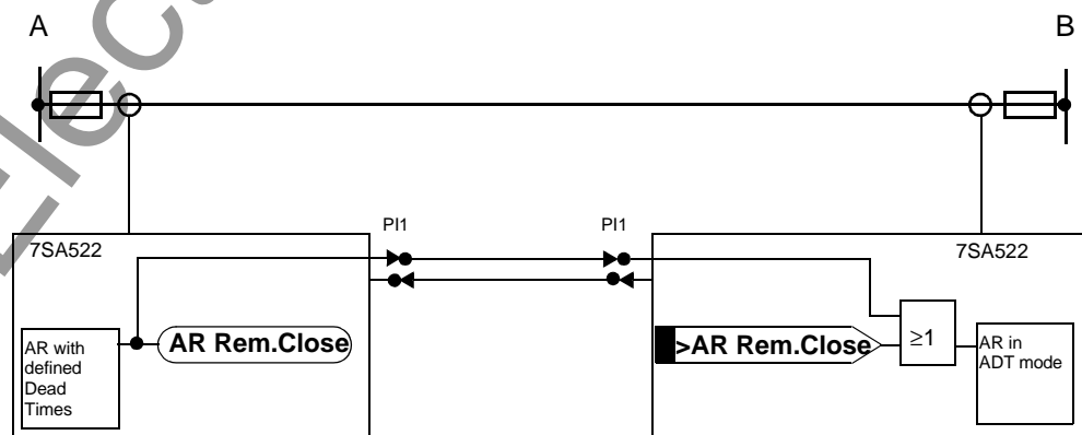
Bild 6-95 AR Remote–Close function via protection interface
