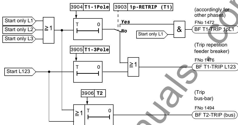
Figure 6-121 Two-stage breaker failure protection with phase segregated initiation — one phase
