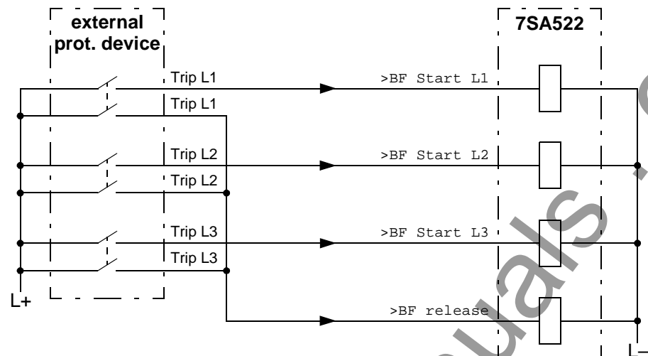
Figure 6-117 Breaker failure protection with phase segregated initiation — example for initiation by an external protection device with release by a separate set of trip contacts
