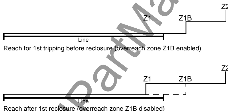
Figure 6-92 Reach control, before the first reclosure, in the distance protection
