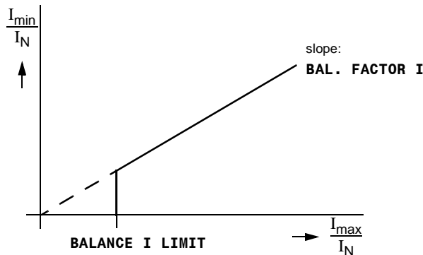
Figure 6-129 Current symmetry monitoring
