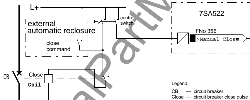
Figure 6-139 Manual closure with external automatic reclosure
