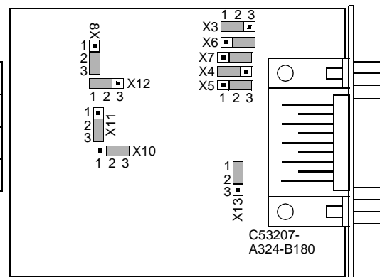
Figure 8-14 Location of jumpers for the configuration of terminating resistors of interface RS485
