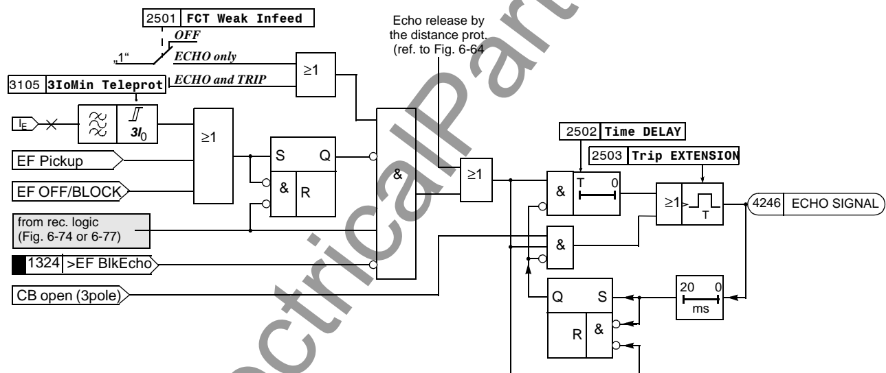
Figure 6-81 Logic diagram of the echo function for the earth fault protection with teleprotection
