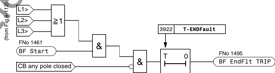
Figure 6-124 Function block diagram of end fault protection
