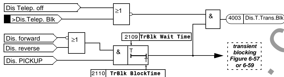
Figure 6-63 Transient blocking with POTT and Unblocking schemes
