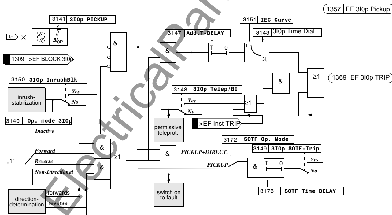
Figure 6-67 Logic diagram of the 3I_{OP} -stage (inverse time overcurrent protection), for example IEC curves
