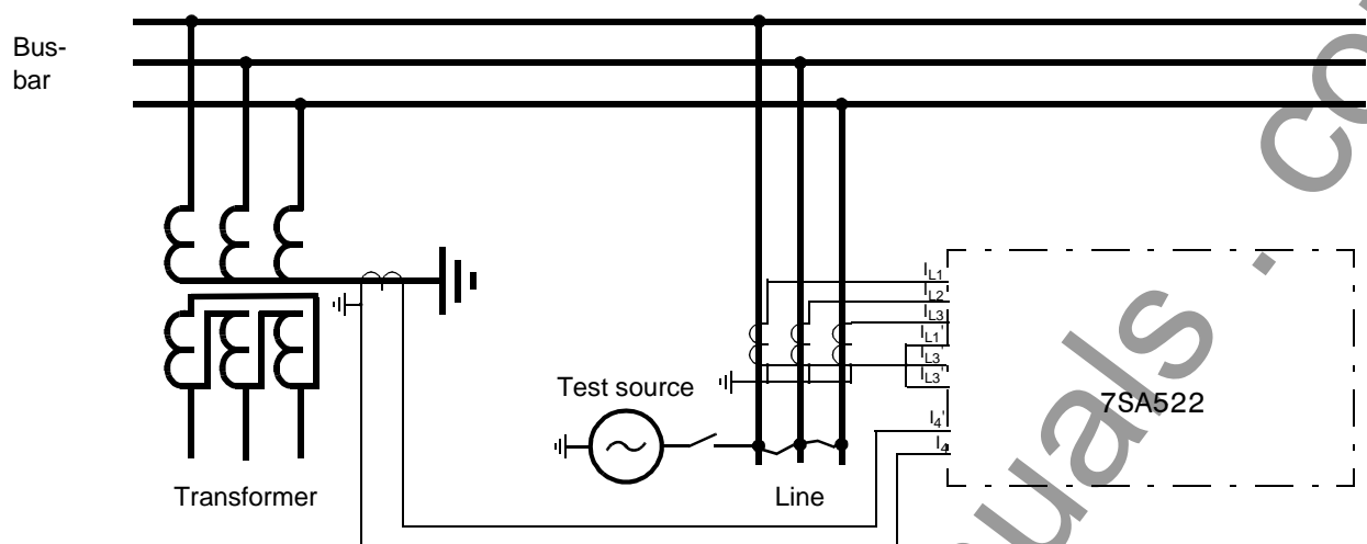
Figure 8-26 Polarity check of I_4 , example with earth current from a power transformer star-point
