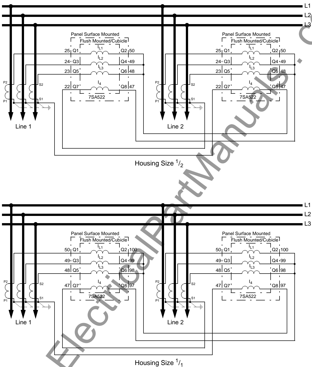
Figure A-17 Current connections to three current transformers but earth current (residual 3I_0 neutral current) from the star-point connection of a parallel line (for parallel line compensation)
