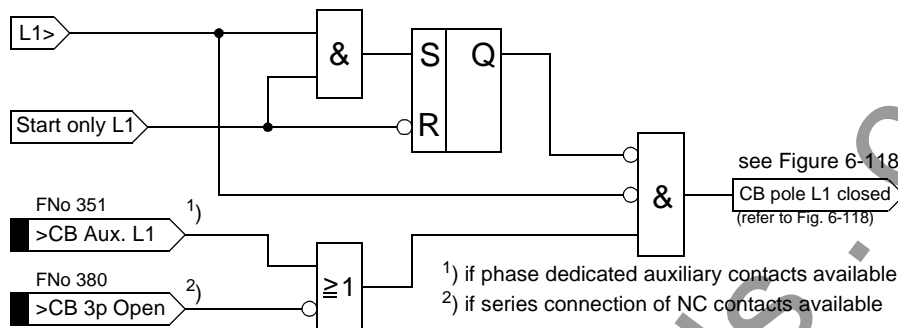
Figure 6-113 Interlock of the auxiliary contact criterion — example for phase L1
