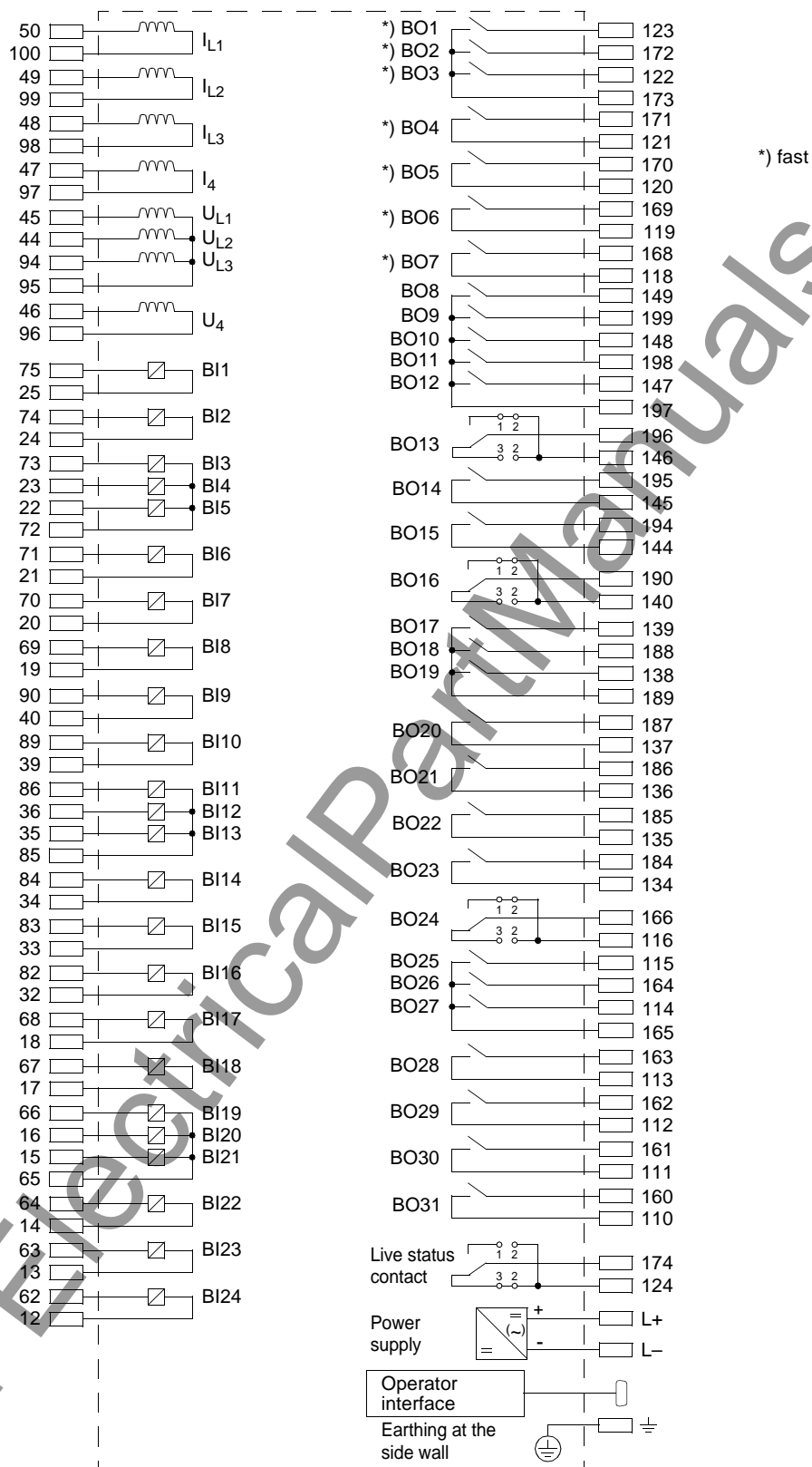
Figure A-11 General diagram 7SA522*—*H (panel surface mounting)
