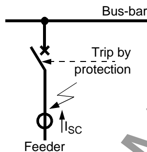
Figure 6-123 End fault between circuit breaker and current transformers
