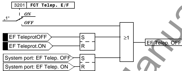
Figure 6-72 Switching on and off of the signal transmission logic
