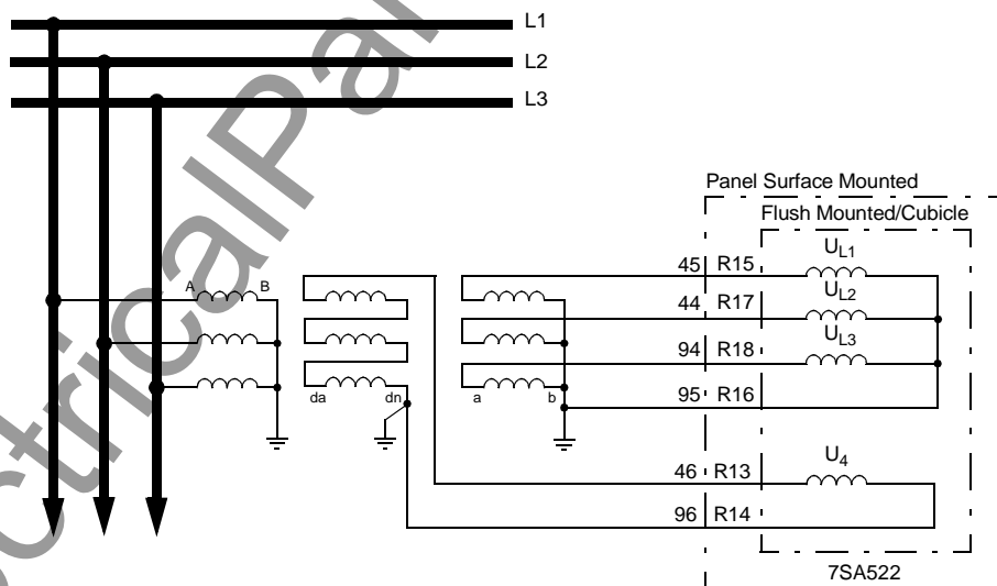
Figure A-20 Voltage connections to three wye-connected voltage transformers with additional open-delta windings (da-dn-winding)
