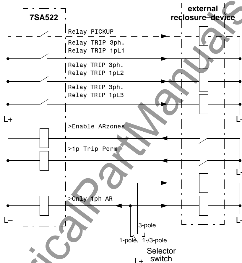
Figure 6-96 Connection example with external reclosure device for 1-/3-pole reclosure with mode selector switch
