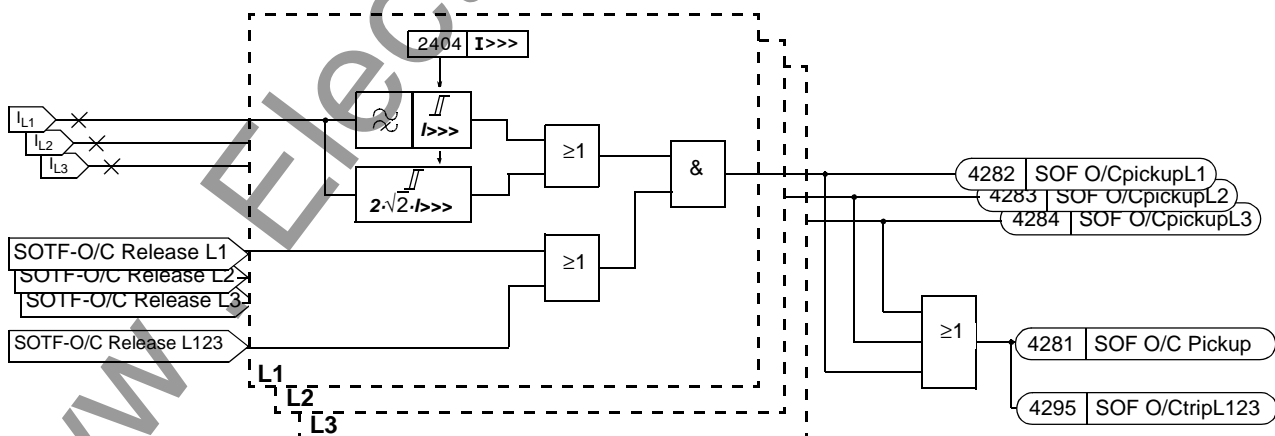
Figure 6-90 Logic diagram of the high current switch on to fault protection
