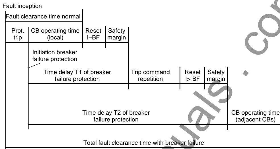
Figure 6-126 Time sequence example for normal clearance of a fault, and with circuit breaker failure, using two-stage breaker failure protection
