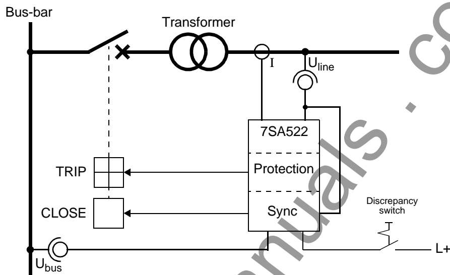
Figure 6-103 Synchronism check across a transformer
