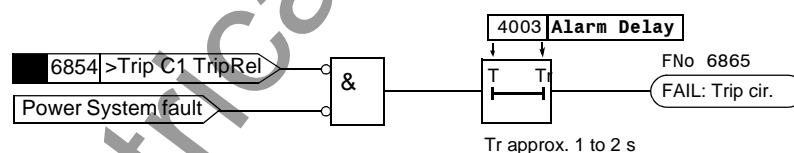
Figure 6-136 Logic diagram of the trip circuit supervision with one binary input
