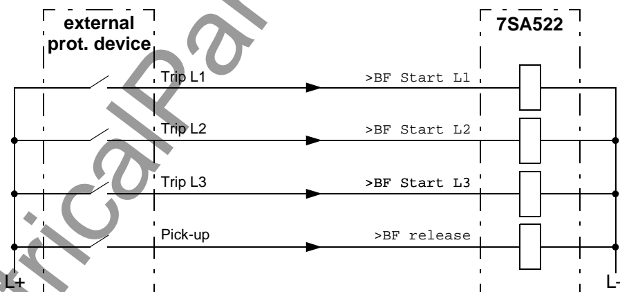
Figure 6-116 Breaker failure protection with phase segregated initiation — example for initiation by an external protection device with release by a fault detection signal
