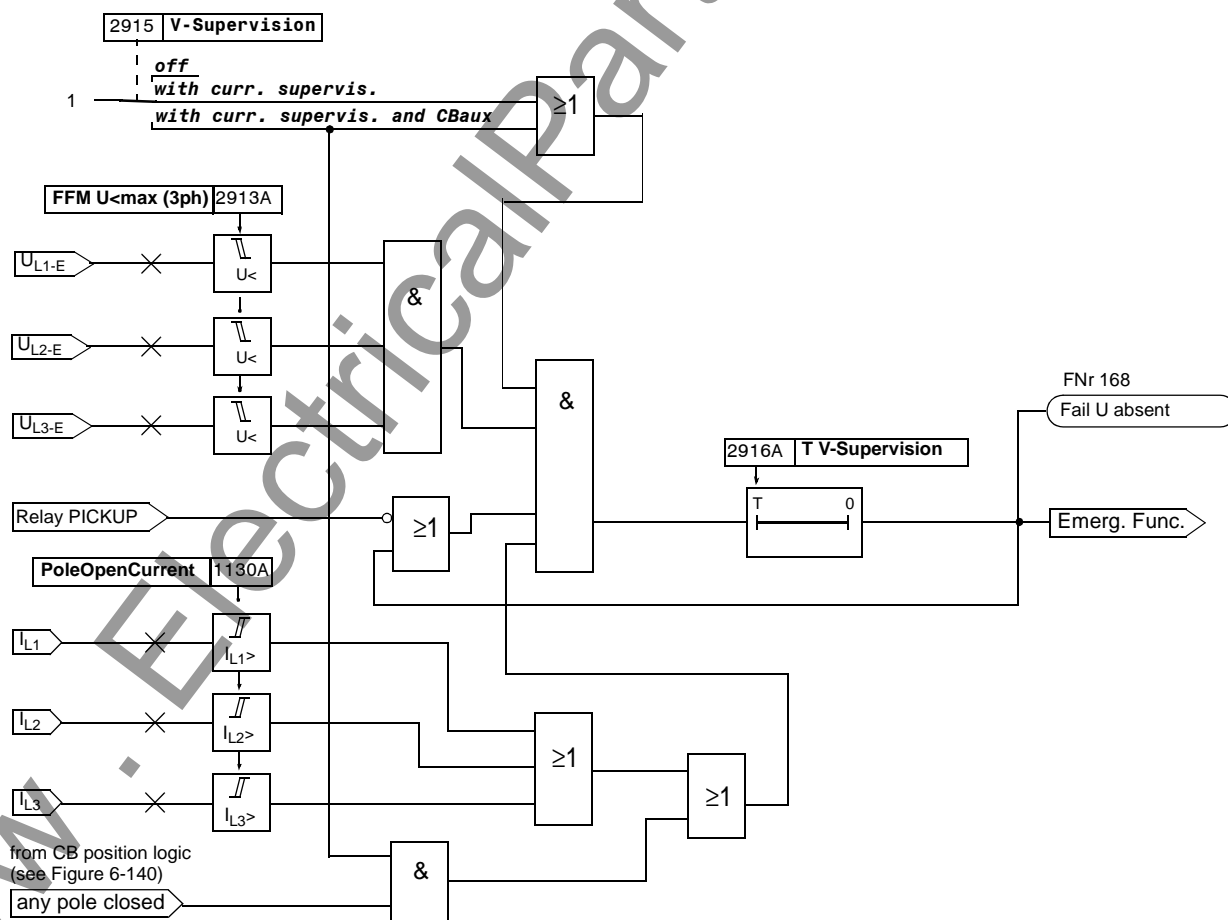
Figure 6-132 Logic diagram of the additional measured voltage failure monitoring
