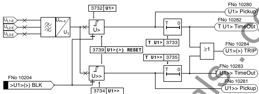
Figure 6-105 Logic diagram of the overvoltage protection for the positive sequence voltage system
