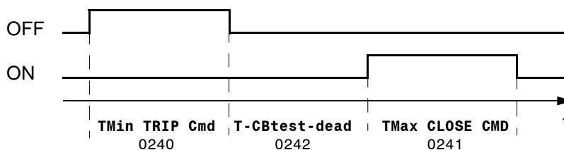
Figure 6-146 Trip/Close test cycle
