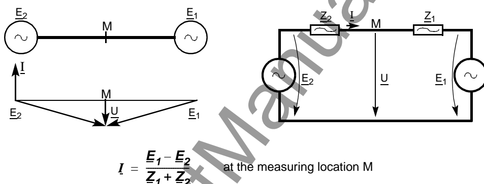
Figure 6-40 Power swing
