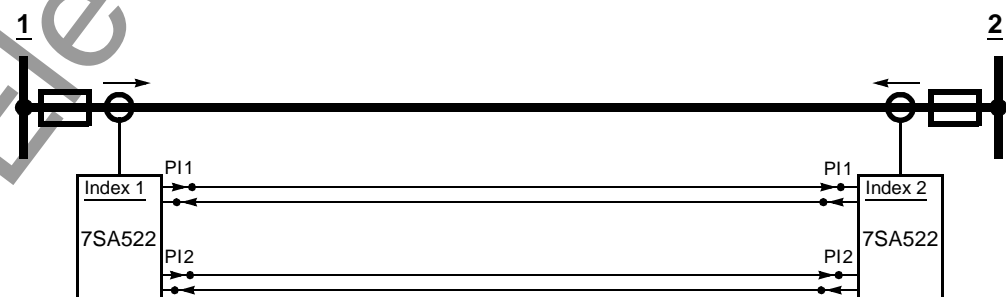
Figure 6-47 Distance Protection for two ends with two 7SA522 devices, each of them having two protection data interfaces (transmitter/ receiver)
