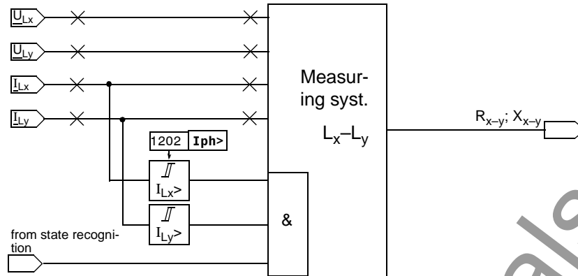
Figure 6-20 logic of the phase-phase measuring system
