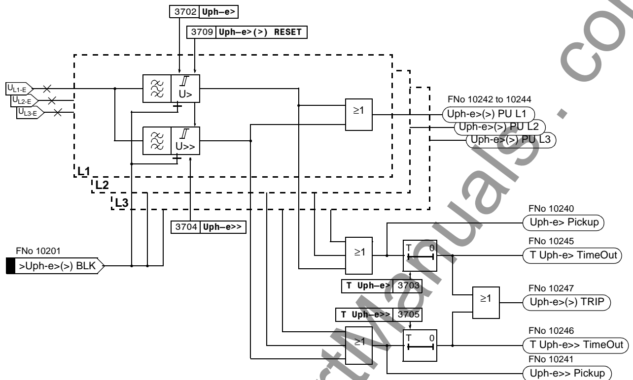
Figure 6-104 Logic diagram of the overvoltage protection for phase voltages
