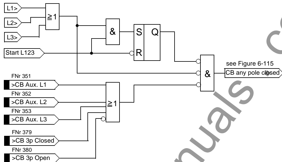
Figure 6-114 Creation process of signal "CB any pole closed"
