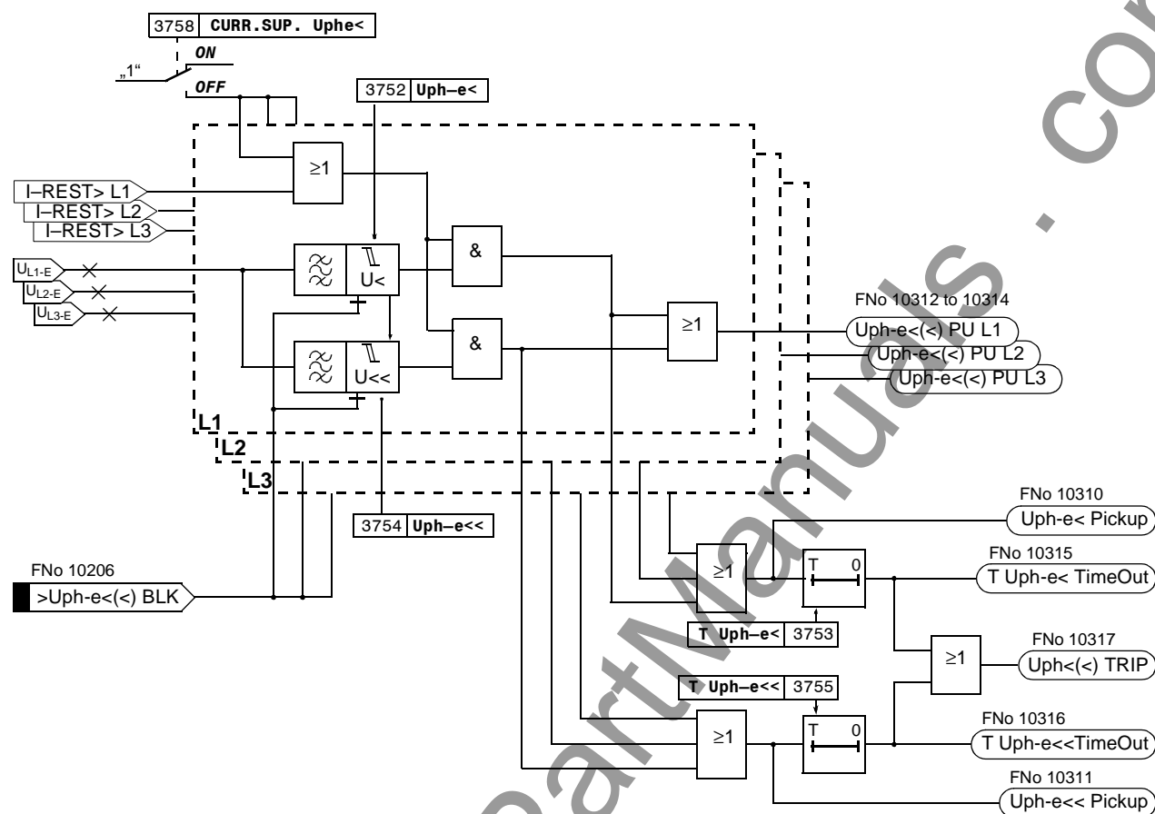
Figure 6-107 Logic diagram of the undervoltage protection for phase voltages
