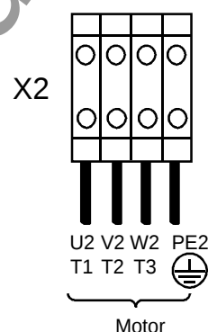
Fig. 3.4 Motor connection
