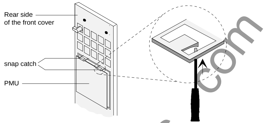
Fig. 8.5 Rear side of the front cover with PMU board
