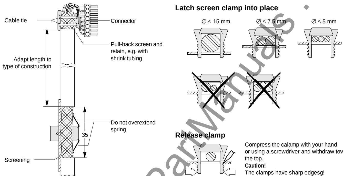
Fig. 3.7 Connecting-up the control cables and the technique for using the screen clamps
