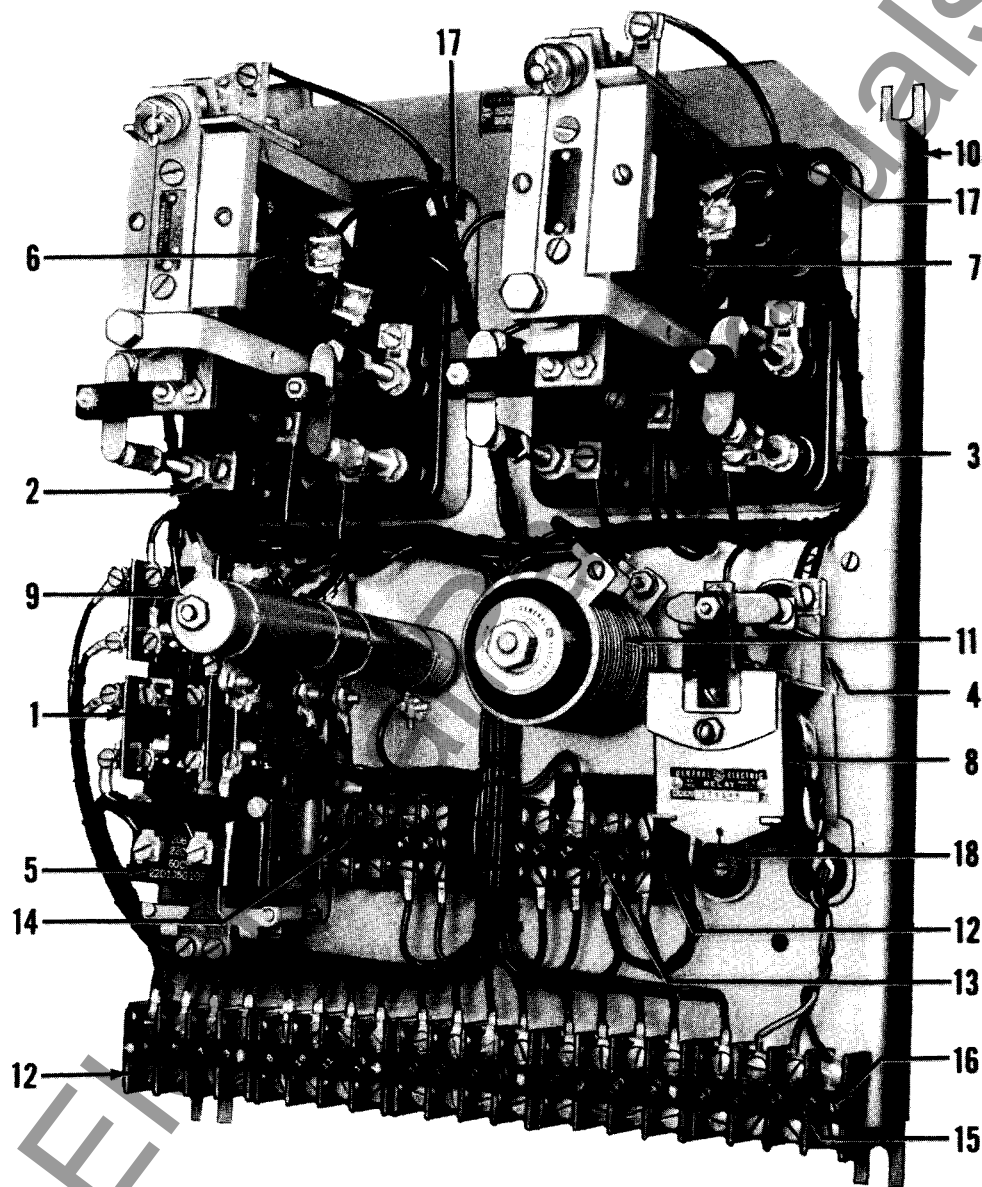
IC7069-B1C Synchronous Motor Field Panel
