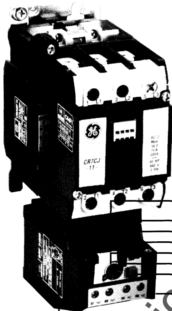
Size J, 40hp Starter with Class 10 Fixed Heater Overload Relay
