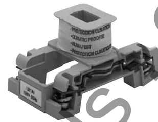
Coil
