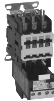
25A-30A with screw terminals and short cover
