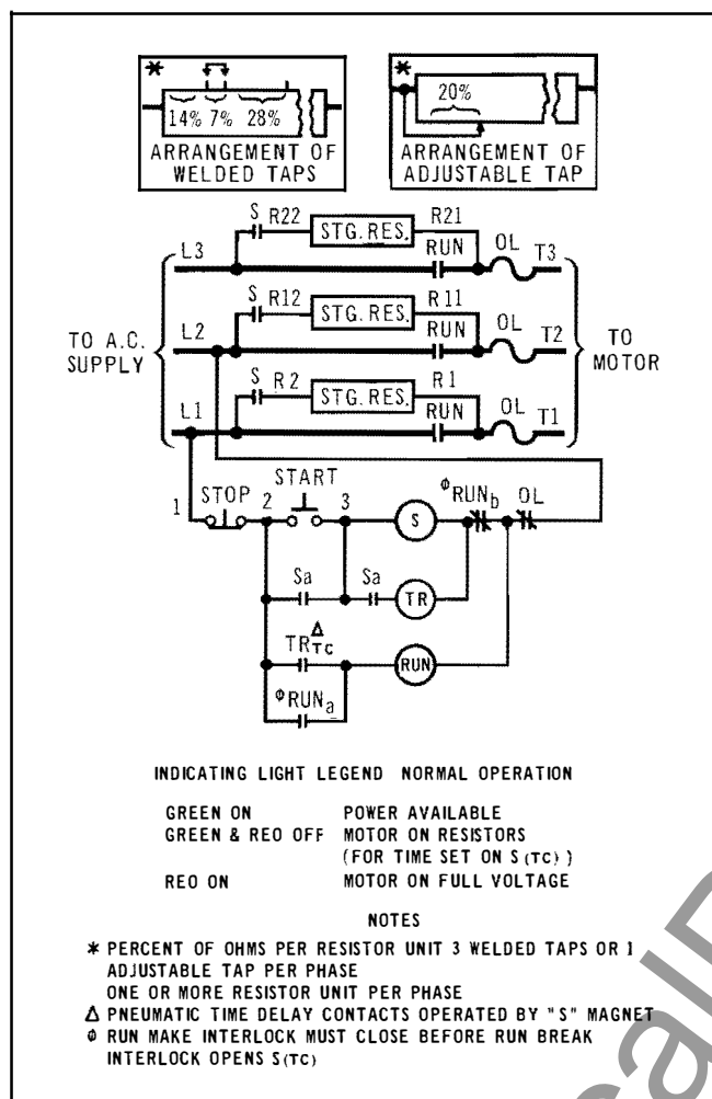
Fig. 1 Typical Elementary Diagram
