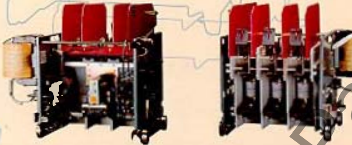
Shown is front view (left) and rear view (right) of new Ampgard Direct Replacement SJ Vacuum Contactor
