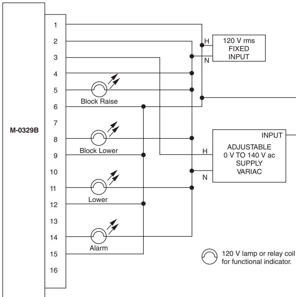
Figure 10 Test Setup
