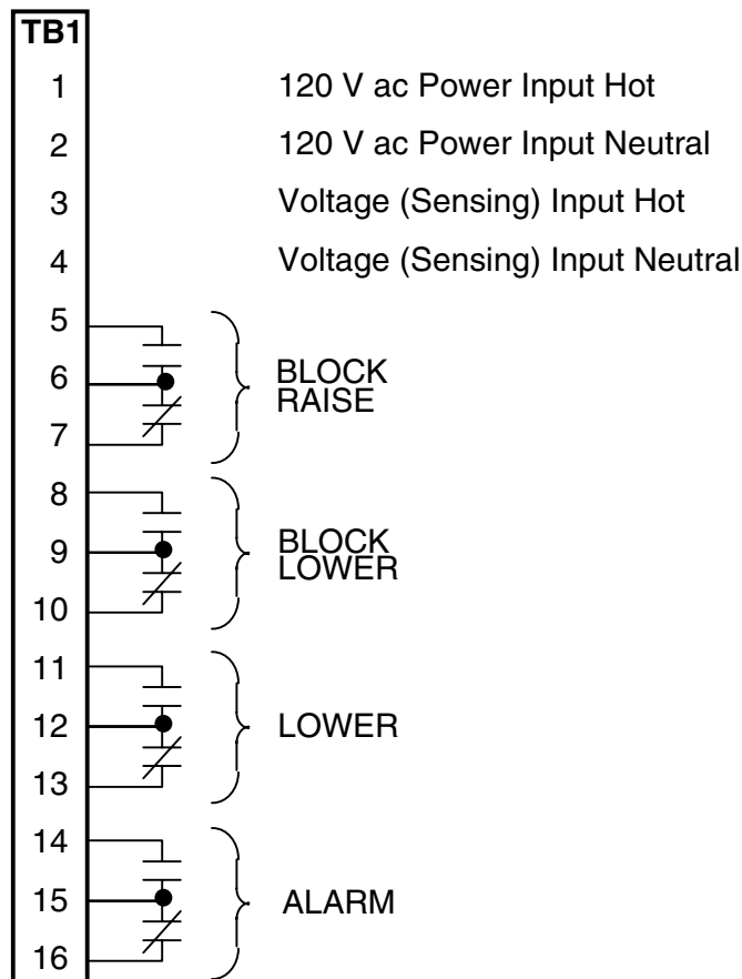
Figure 3 Wire Terminations for External Connections as Required for UL Listing
