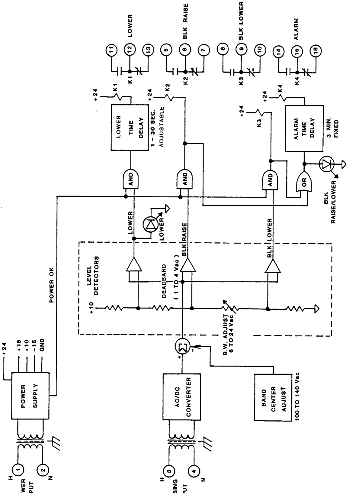
Figure 9 Block Diagram
