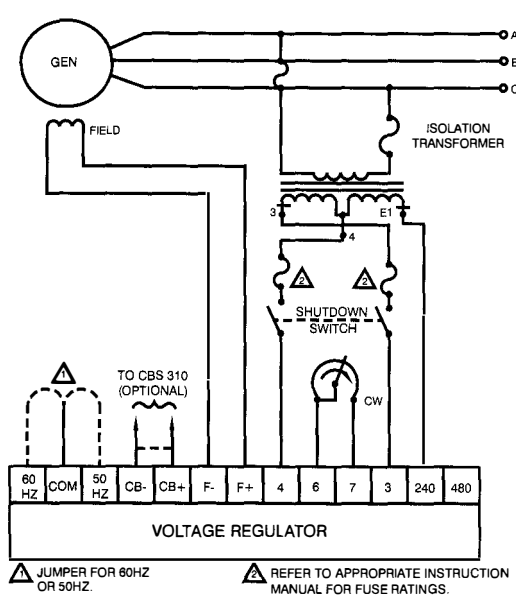
Figure 5 - Typical Interconnection
