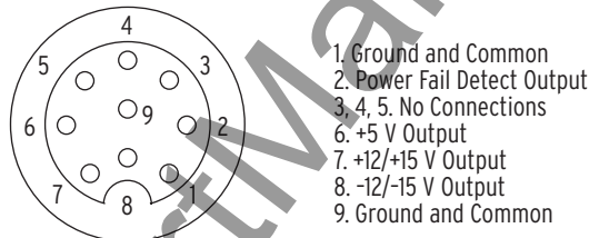
Figure 1 Female Chassis Connector, Exterior View
