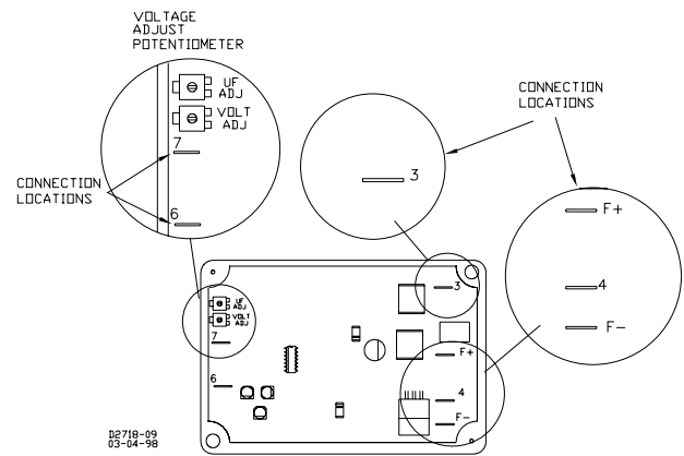
Locations of Controls and Connectors
