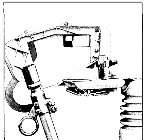
4. Further opening of the cutout releases the C-blade and it snaps the length of the arc chute elongating and deionizing the arc. This action insures safe loadbreak operation independent of the operating speed of the lineman.
