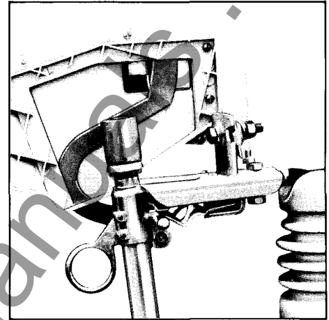
2. As the cutout is pulled open, the C-blade becomes a current path before the main contacts part. This eliminates arcing and pitting of the main contacts.
