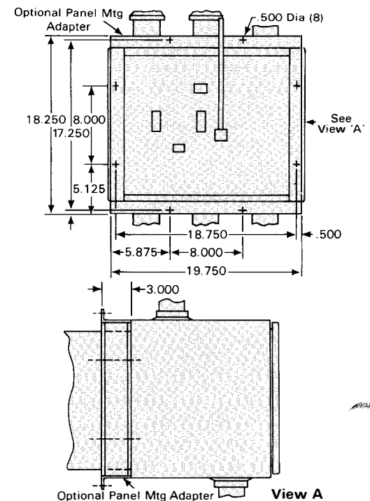
Figure 5 Panel Mounted MVB-5 ① Opposite Bushing Location With Optional Panel Adapter O.D. 1883B19
