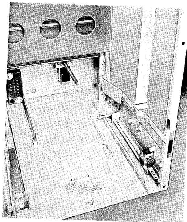
Fig. 22. Indoor and Outdoor: Close-up, Position Interlock (Locked)
