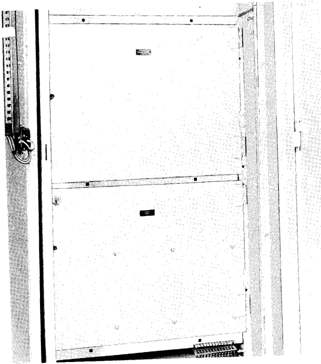
Fig. 25. Indoor and Outdoor: 15 KV Auxiliary Housing with PT and Fuse Doors Closed
