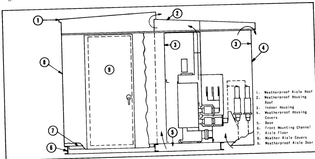
Fig. 6. Shelterfor-M: 5 KV Breaker Housing*
