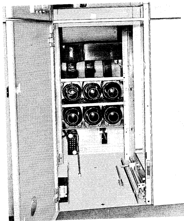
Fig. 20. Indoor and Outdoor: 5 KV Breaker Housing with Shutter and Barriers Removed
