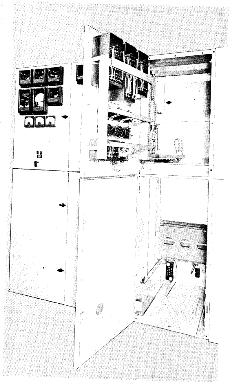
Fig. 16. Indoor and Outdoor: 5 KV Breaker Housing with PT Compartment Door Closed
