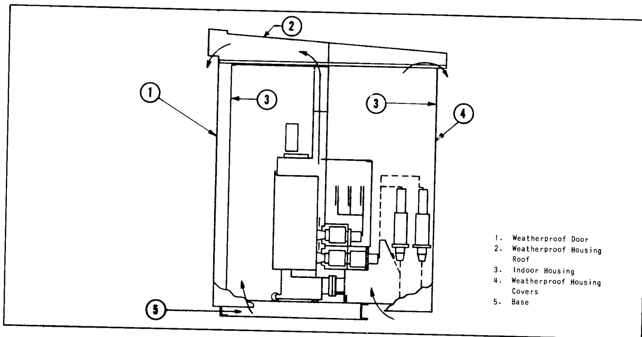
Fig. 7. Aisle-less: 5 KV Breaker Housing (Ventilation indicated by arrows)
