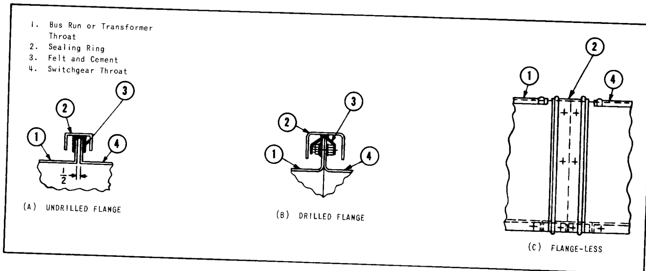
Fig. 41. Sealing Rings for H.V. Enclosures
