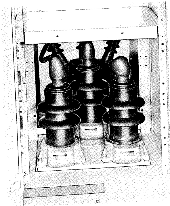
Fig. 27. Indoor and Outdoor: Lightning Arresters
