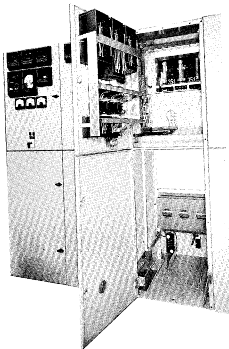
Fig. 17. Indoor and Outdoor: 5 KV Breaker Housing with PT Compartment Door Open
