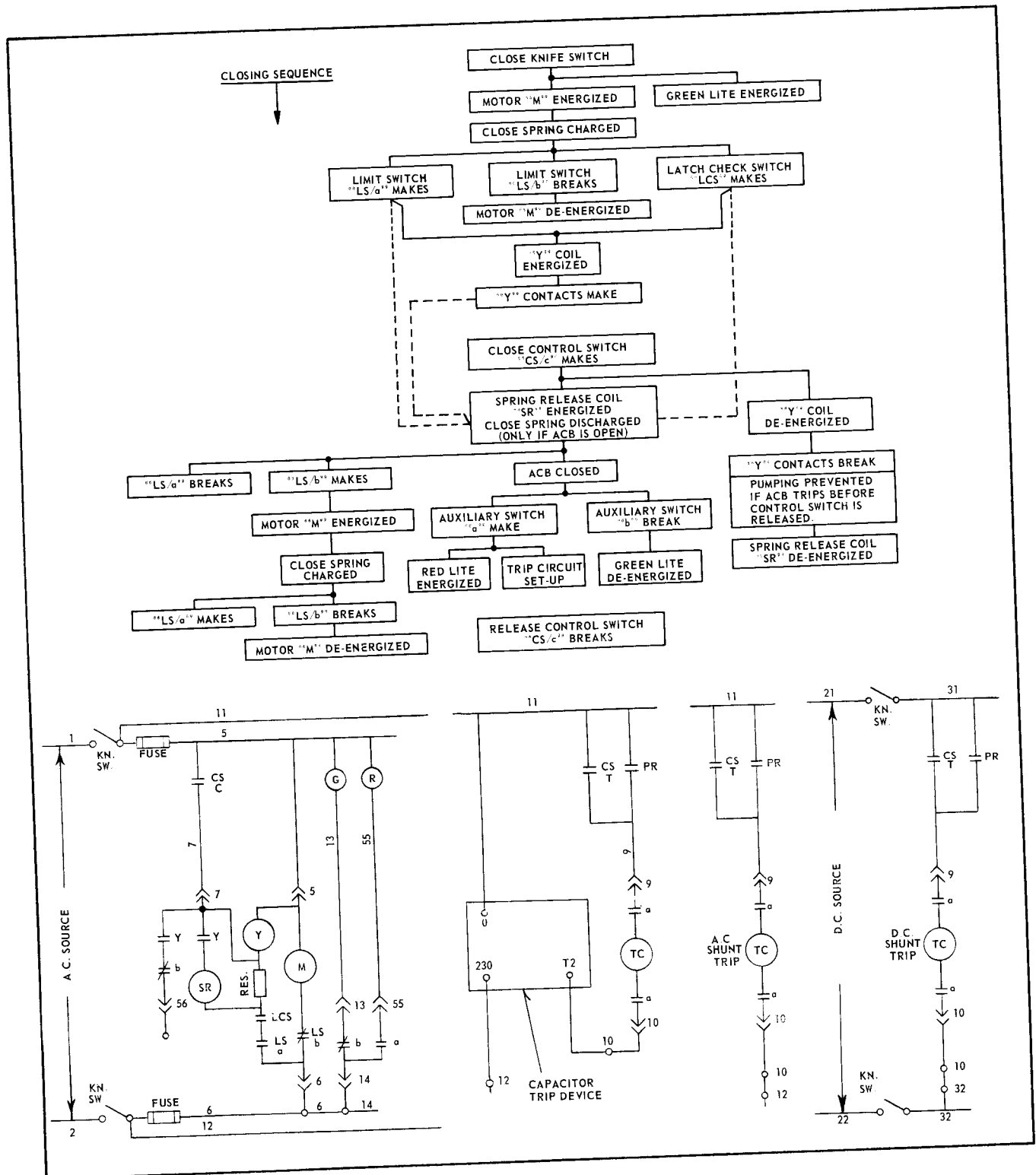
Fig. 45. Stored Energy Breaker with AC Control and Alternate Tripping Schemes
