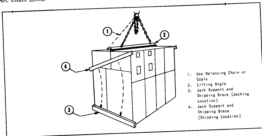
Fig. 39. Handling of Indoor Shipping Group
