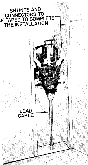
Fig. 42. Typical Main Cable Installation
