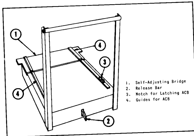
Fig. 36. Transport Truck
