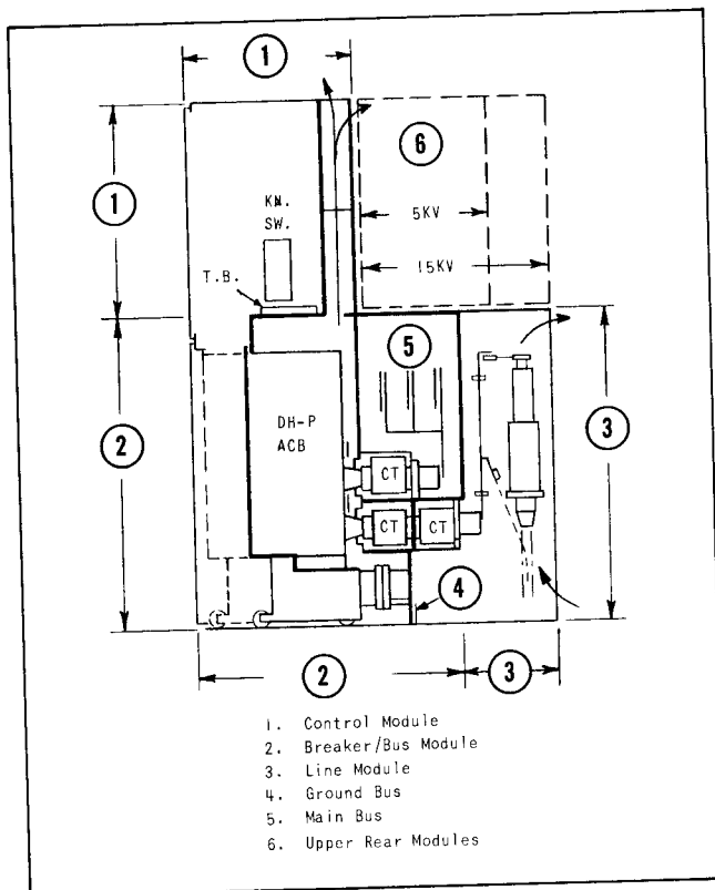
Fig. 4. Indoor: 5 KV Breaker Housing*
