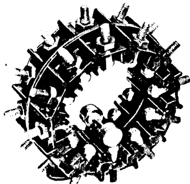
12 Contact Frame With Overlapping Contact Roller (Make Before Break)
