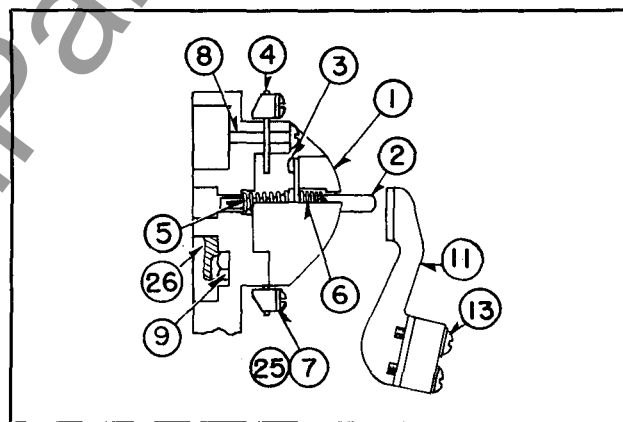
FIG. 5. Renewal Parts Item Numbers
