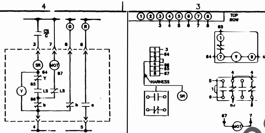
PWR OPR MECH W/O SHUNT TRIP 15A
