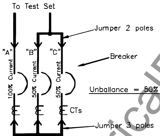
Figure 10.1 U/B Test
