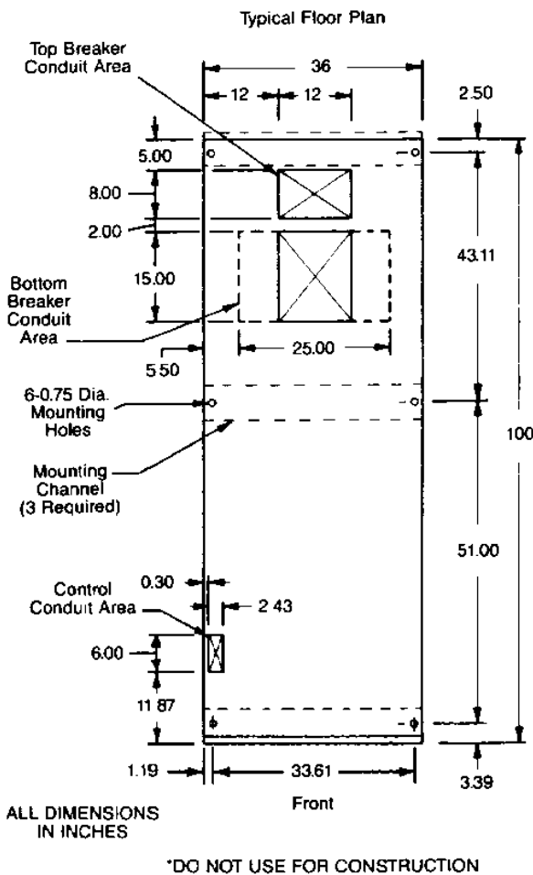
FLOOR PLAN (Typical two breaker combination)
