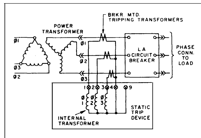
Figure 5. — Breaker Wiring for Types T1, TS, and TSI (non ground)
