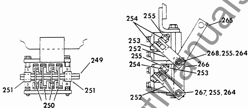
FRONT VIEW COVER REMOVED
