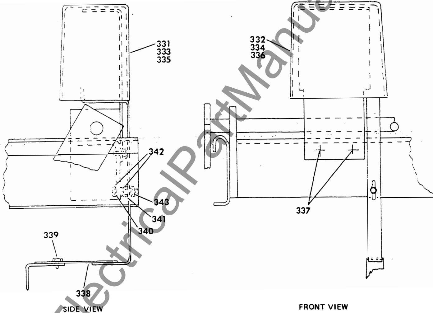
Figure 10. LA-600A/800A/1600A Undervoltage Trip Group
