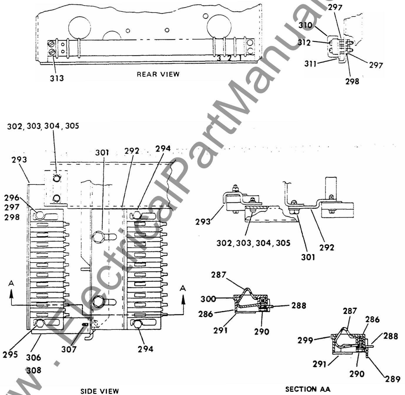
Figure 9. LA-600A/800A/1600A Secondary Disconnect Group
