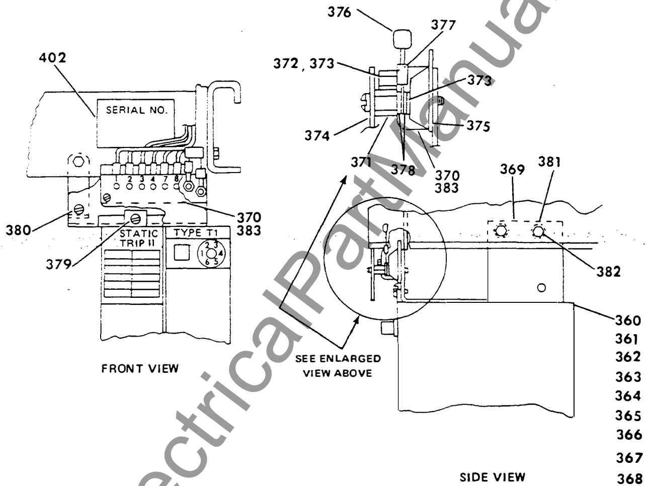
Figure 11. Static Trip Group
