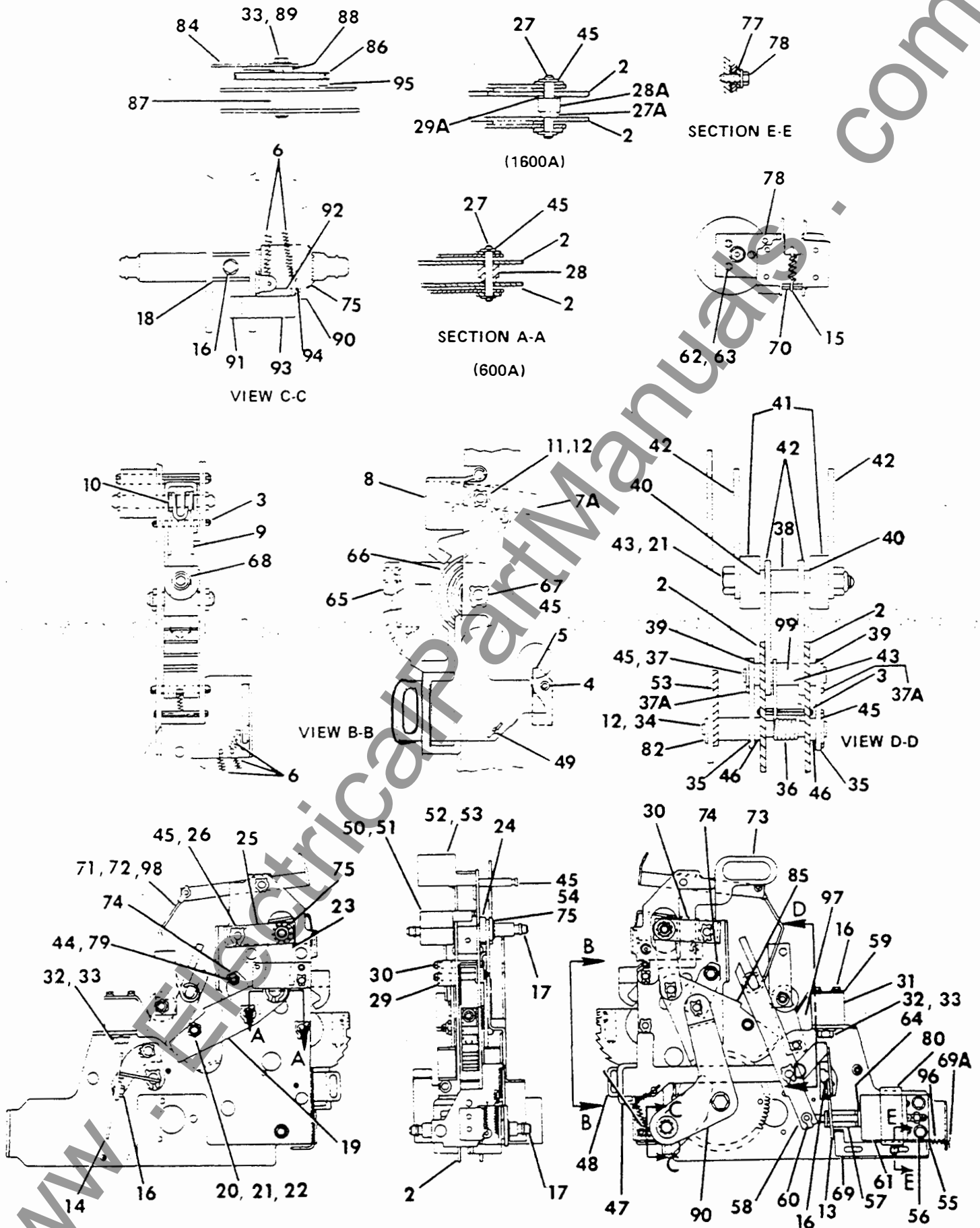
Figure 3. LA-600A/800A/1600A Operator
