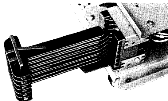
Fig. 8—Secondary Disconnecting Device
