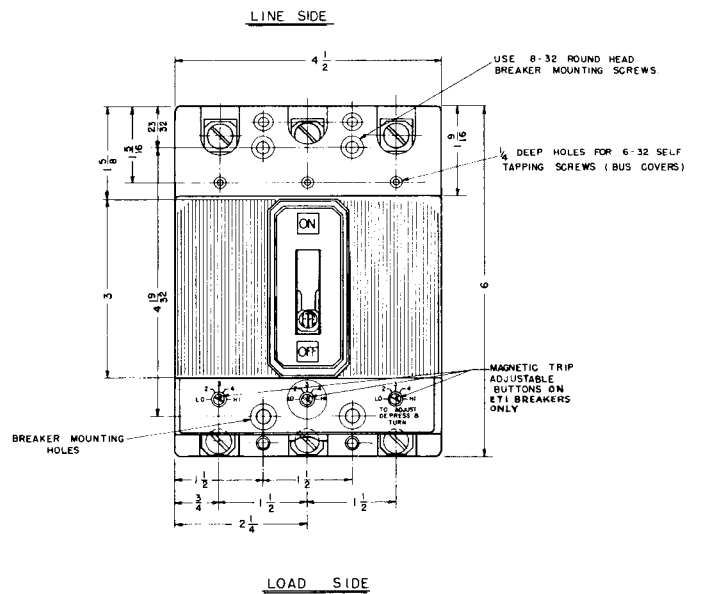
100-Ampere ETI EF-Frame Circuit Breakers Dimensional Drawings
