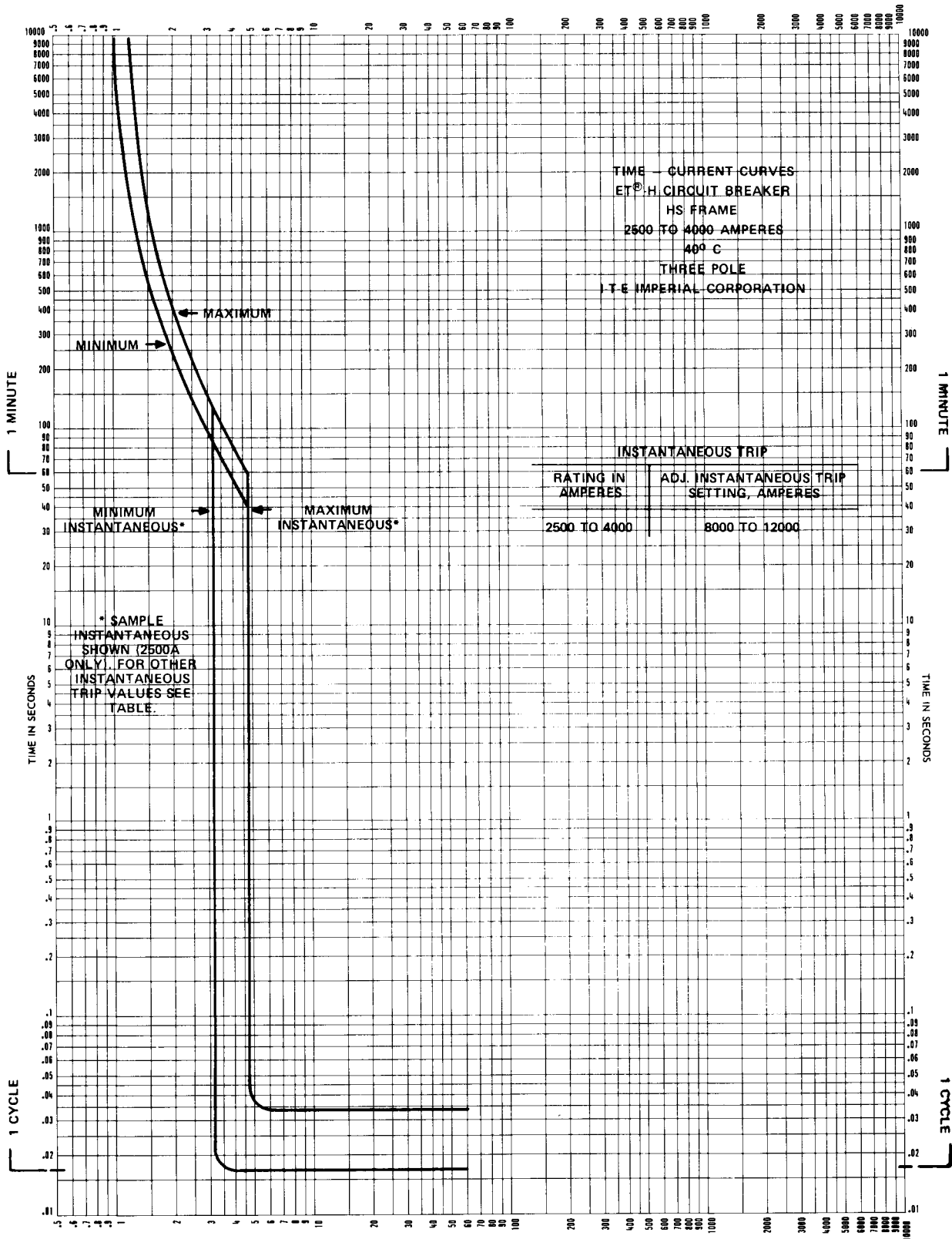
MULTIPLES OF CIRCUIT BREAKER CURRENT RATING
