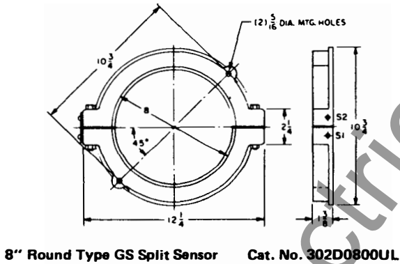
8" Round Type GS Split Sensor Cat. No. 302D0800UL
