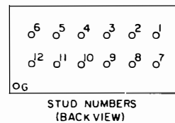
Figure 3—Semi-Flush Mounted Relay—Outline and Drilling
