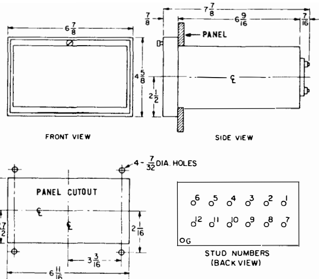
Figure 3—Semi-Flush Mounted Relay—Outline and Drilling
