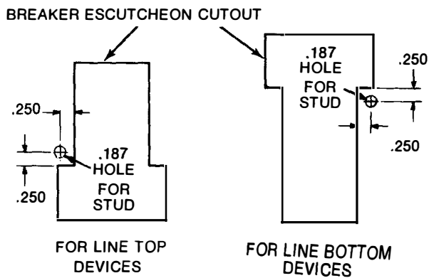
Figure 5. Door drilling for Versatrip and Selectrip Breakers
