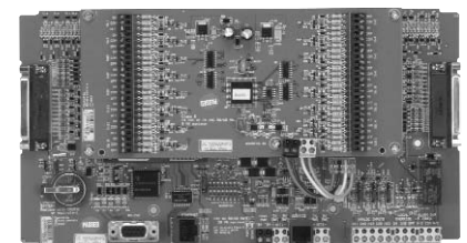
Controller
