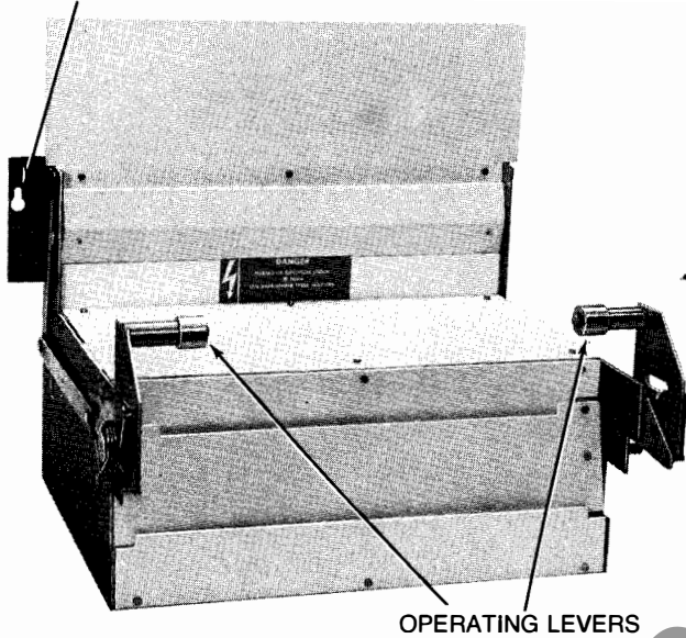
Figure 12 Fused unit shutter
