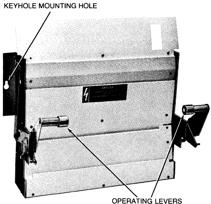
Figure 11 Non-fused unit shutter
