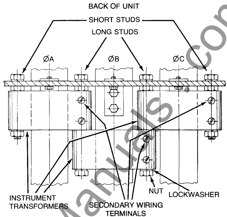
Figure 10 Top partial view of load conductors
