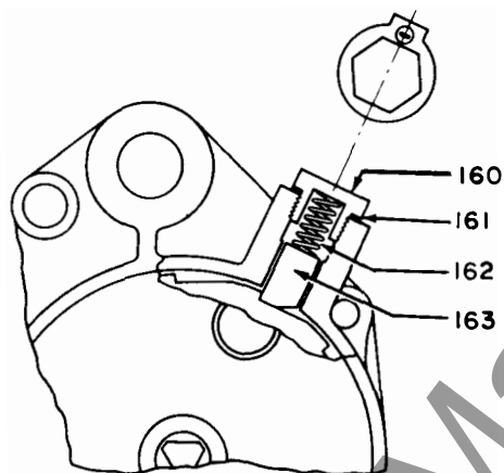
Fig. 9. Section of gear box.
