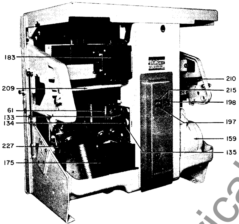
Fig. 14. Type AK-2A-75 power circuit breaker.
