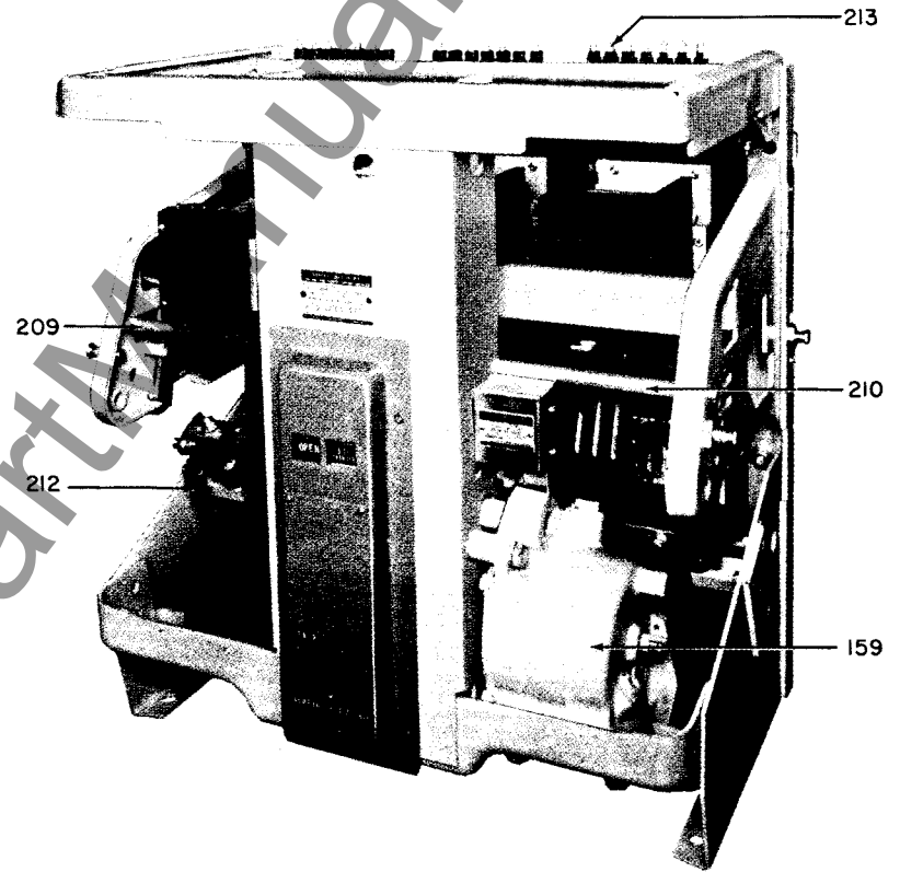
Fig. 15. Type AK-2A-75 power circuit breaker.
