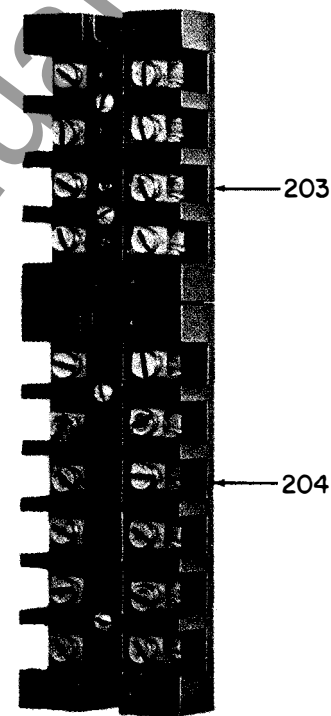
Fig. 17. Terminal boards, without cover.
