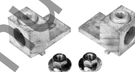
PowerMark Gold main lug kits - TMLK200
