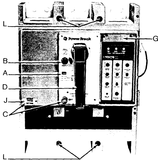
FIG. 4 MANUAL CHARGE MICRO VERSATRIP®
