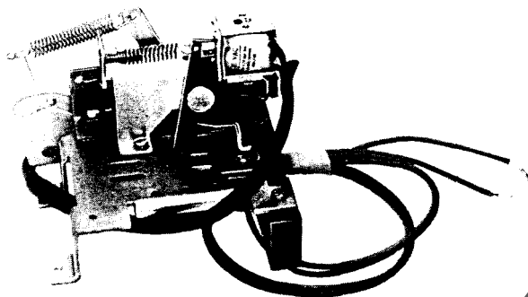
FIG. 29. UNDERVOLTAGE RELEASE ACCESSORY SHOWN ASSEMBLED TO MOUNTING PLATE
