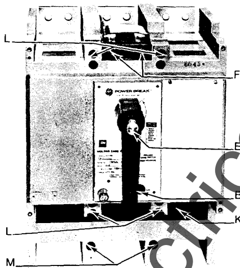
FIG. 5 ELECTRICAL CHARGE MOLDED CASE SWITCH
