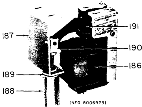
Fig. 15. Time-delay undervoltage tripping device
