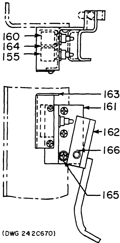
Fig. 12. Motor cut-off switch
