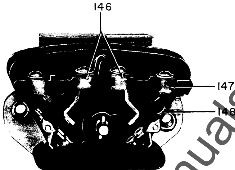
Fig. 11. Type SB-12 auxiliary switch, with back frame removed
