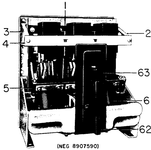
Fig. 2. Manual breaker, front view
