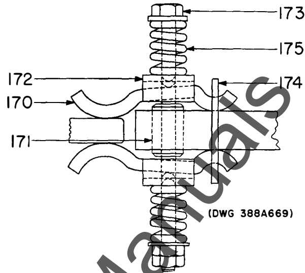
Fig. 13. Primary disconnect
