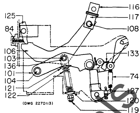
Fig. 8. Electrically operated mechanism
