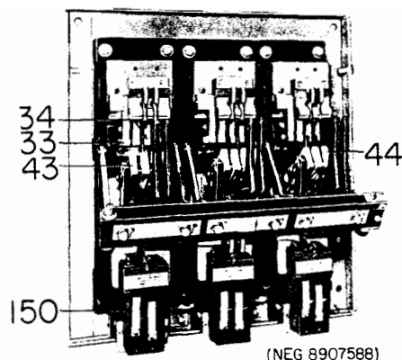
Fig. 6. Back frame assembly, front view
