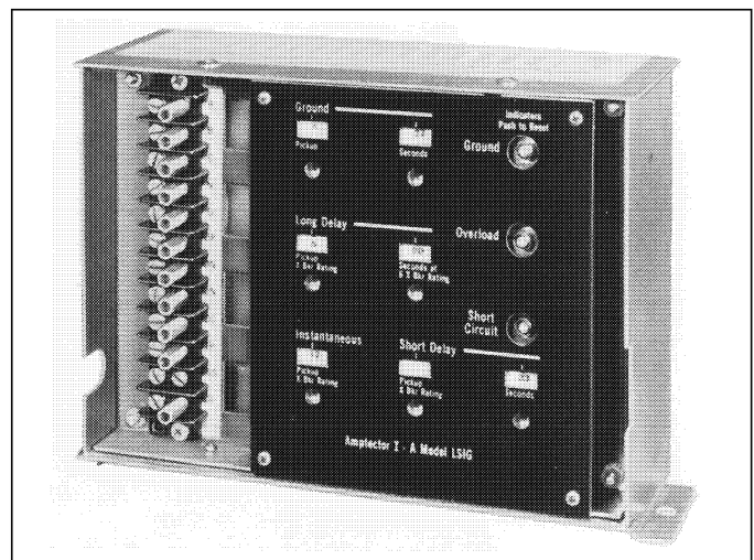
Fig. 62 Optional Amptector I-A Solid-State Trip Unit (396707)
