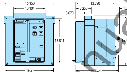
800-3200 Ampere Frame
