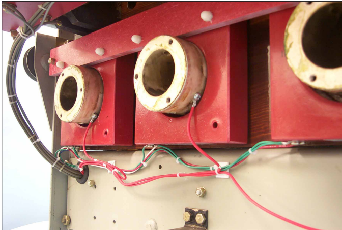
Fig. 23 PT Wires Attached to the Breaker Connectors.
