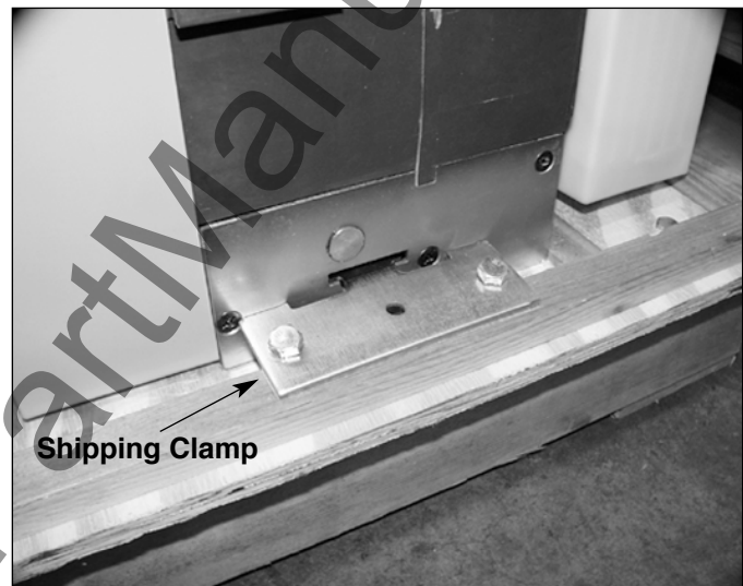
Figure 2-1 Shipping Clamps for Drawout Circuit Breaker
