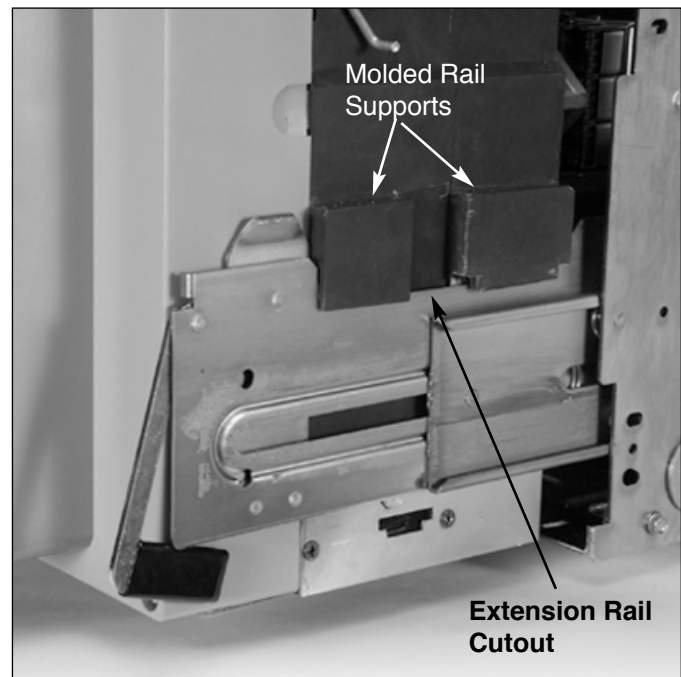
Figure 2-4 One Side of Drawout MDS/MDSX Circuit Breaker Properly Seated on Extension Rail
