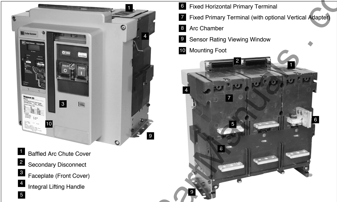
Figure 3-2 Typical MDS/MDSX Fixed Circuit Breaker Features (Front and Rear Views) (MDSX shown without required arc hood)
