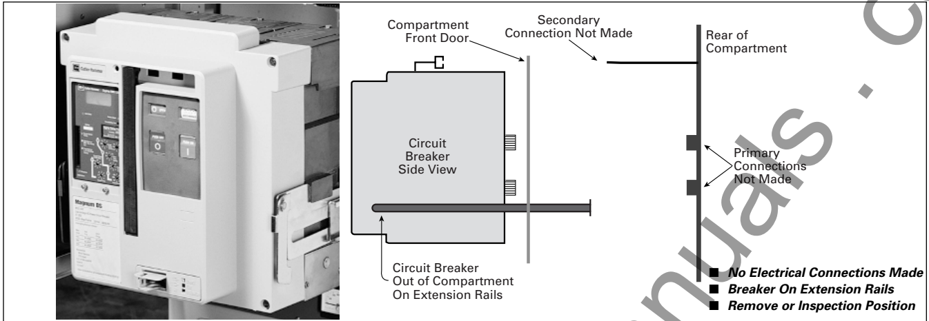
Figure 2-6 Remove Position
