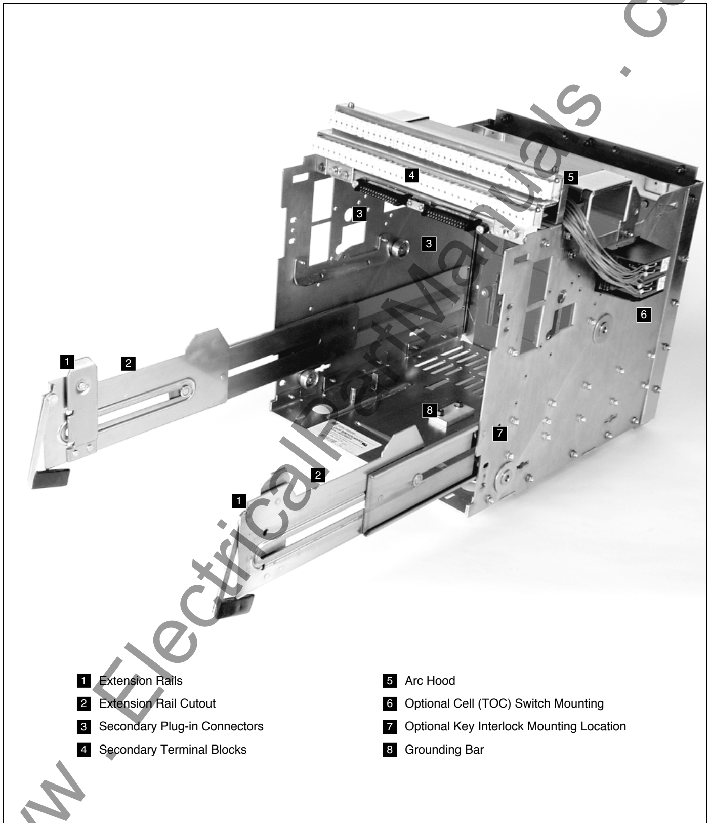
Figure 4-3 Typical Drawout Cassette Features
