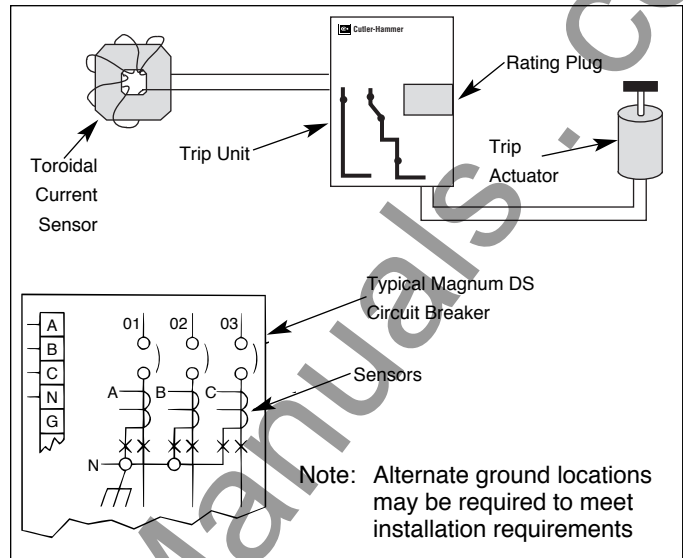
Figure 3-17 Pictorial Diagram of Typical Current Sensing, Processing and Tripping System
