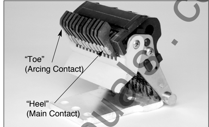
Figure 3-9 Standard Frame DS (12-finger) Moving Conductor Assembly
