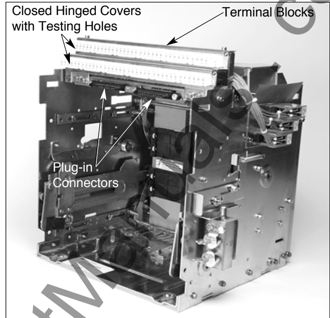
Figure 3-24 Typical Cassette Mounted Secondary Wiring
