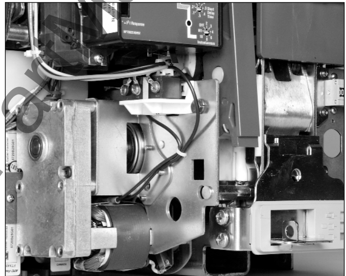
Figure 3-56 Motor Operator Installed in Narrow Frame Circuit Breaker
