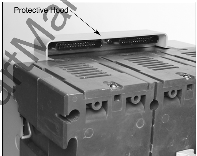
Figure 3-23 Secondary Connector Protective Hood
