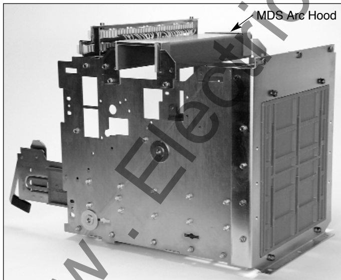
Figure 4-6 Typical MDS/MDSX Basic Cassette (Without Stabs) (Shown with MDS Type Arc Hood)
