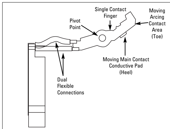
Figure 3-7 Features of Magnum Moving Conductor Assembly
