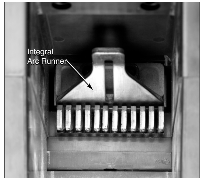
Figure 3-15 Integral Arc Runner Viewed From Top of Arc Chamber (Arc Chute Removed, Circuit Breaker Closed)
