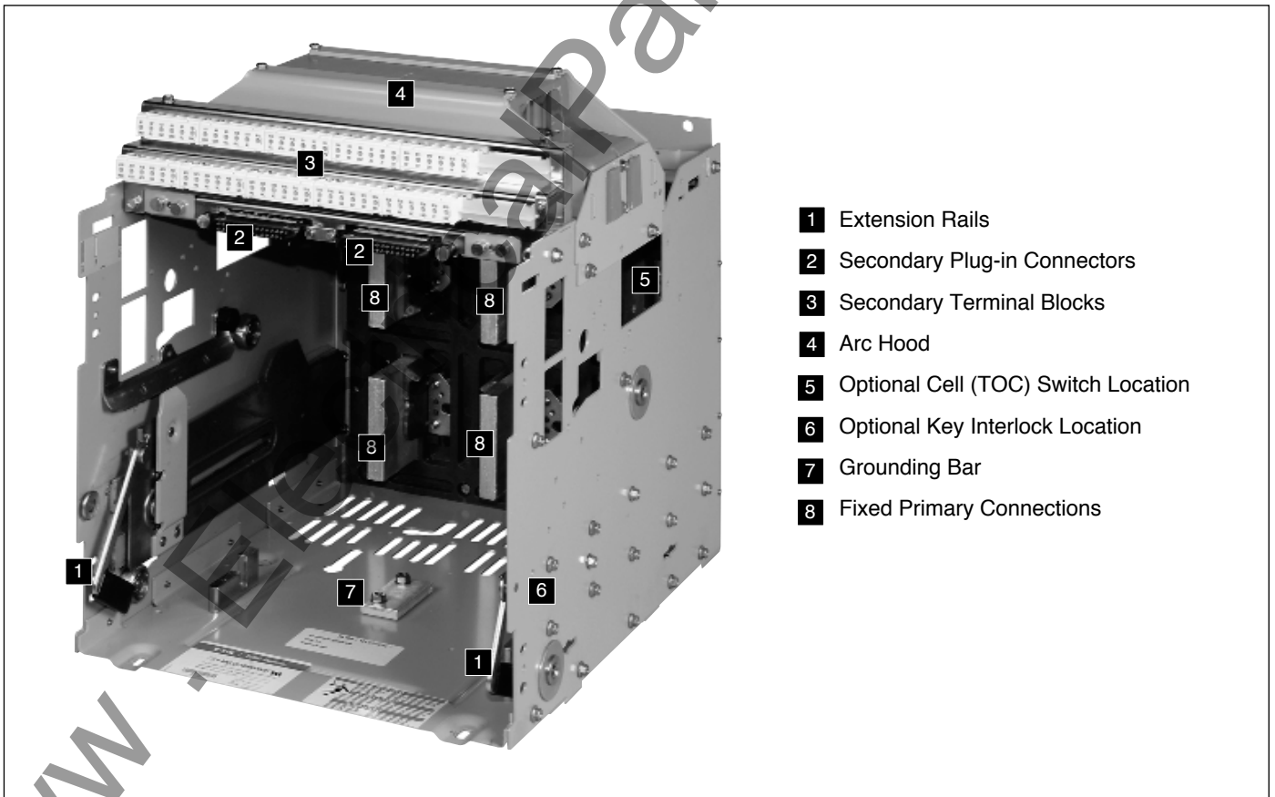
Figure 4-10 Typical MDSX Type Drawout Cassette
