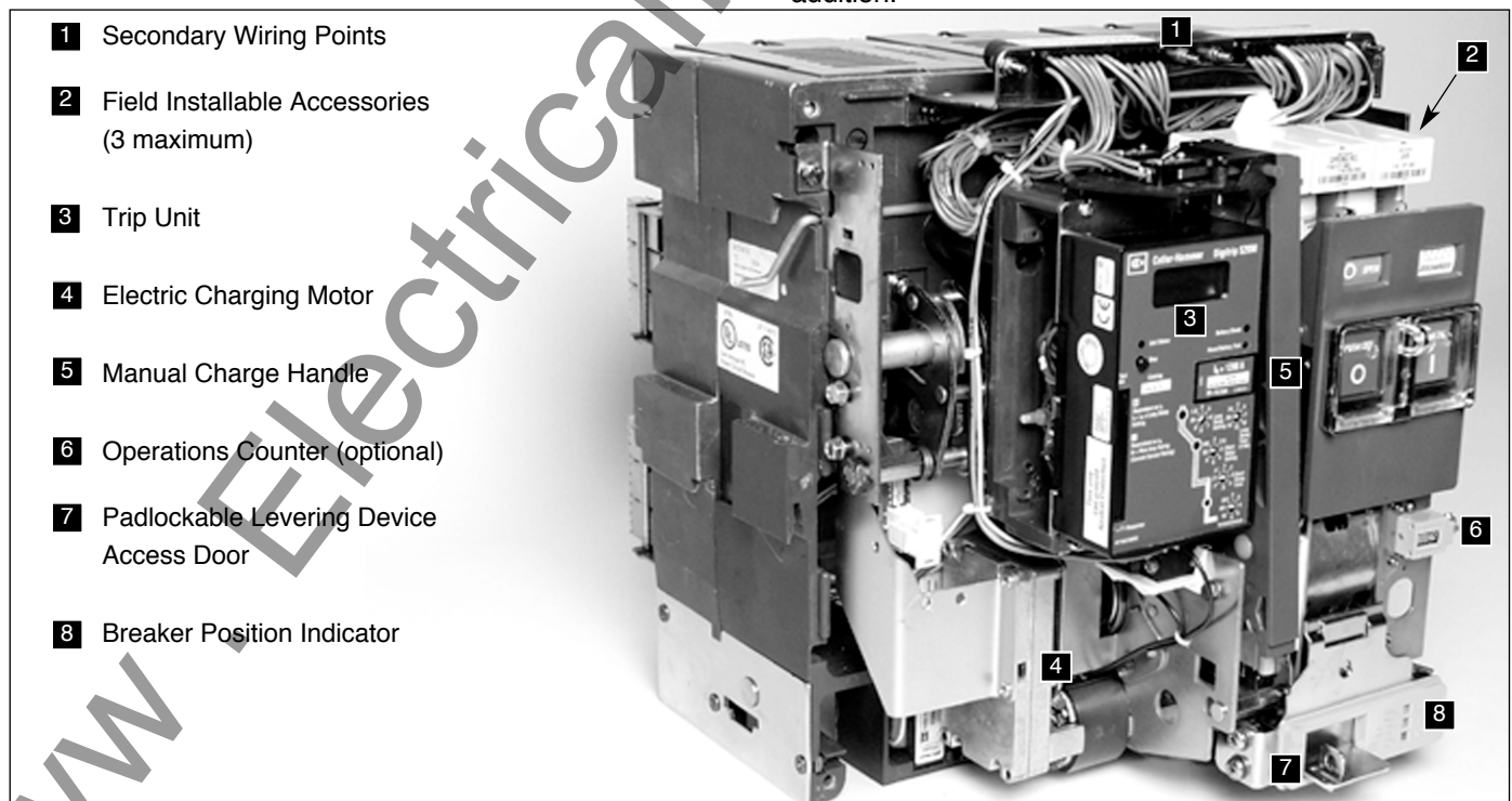
Figure 3-11 Typical Electrically Operated Drawout MDS/MDSX Circuit Breaker with Front Cover Removed
