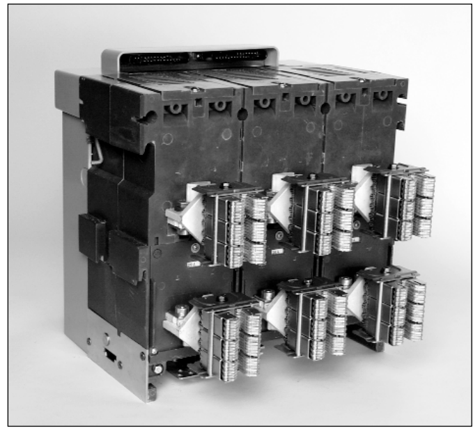
Figure 4-2 MDS/MDSX Drawout Circuit Breaker with Automatic Primary Disconnects
