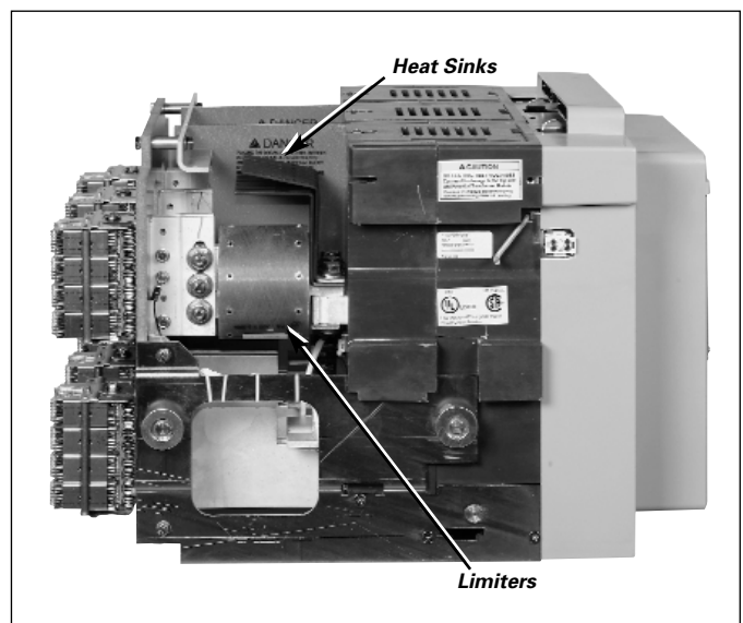
Figure 6-9 MD Limiters Shown Mounted in Extension
