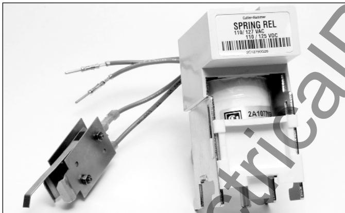
Figure 3-50 Spring Release with Optional Latch Switch
