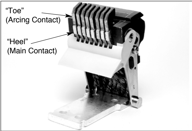
Figure 3-8 Narrow Frame (8-finger) Moving Conductor Assembly
