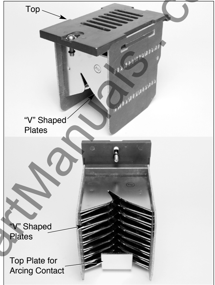
Figure 3-16 Magnum Arc Plate Assembly
