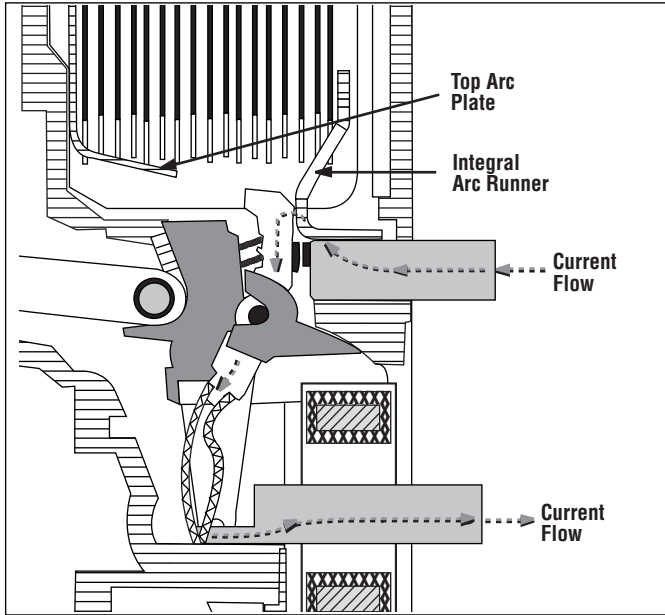
Figure 3-14 Cross Section of Conductor and Arc Control System
