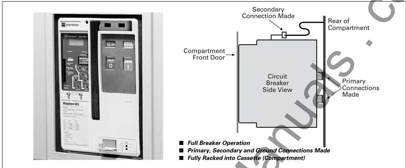
Figure 2-9 Connect Position
