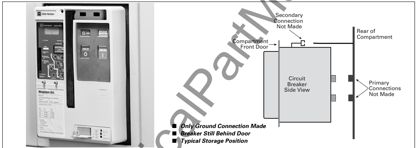
Figure 2-7 Disconnect Position
