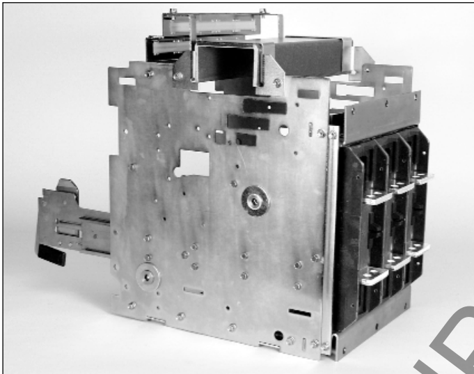
Figure 4-4 Typical MDS Narrow Frame Cassette (Horizontal Terminals)
