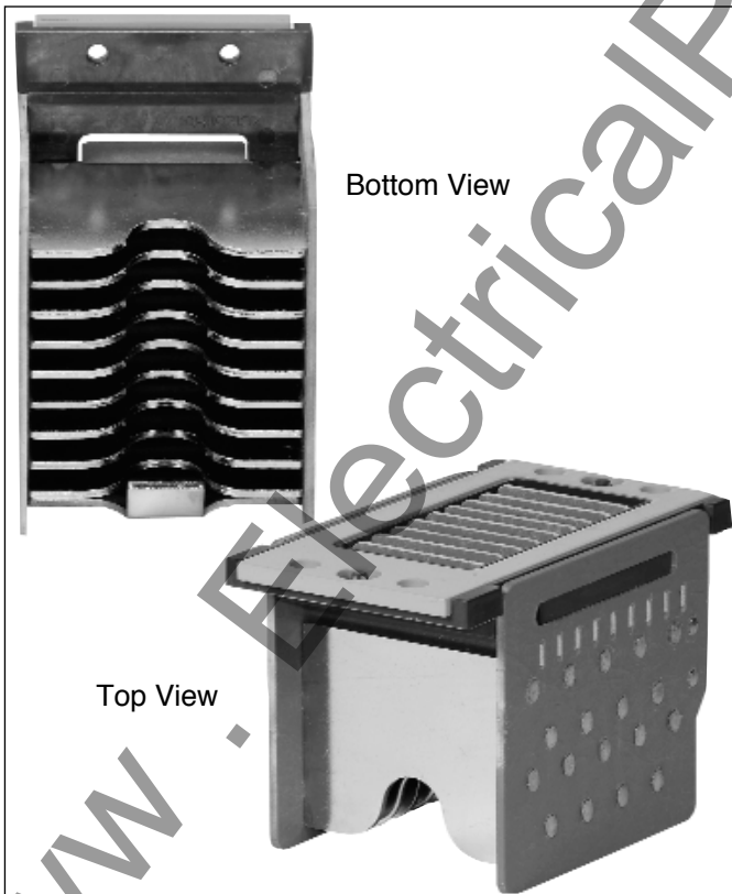
Figure 3-16a Magnum DSX Arc Chute
