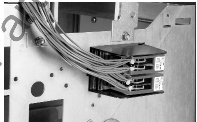
Figure 3-63 Cell Switches Mounted on Cassette
