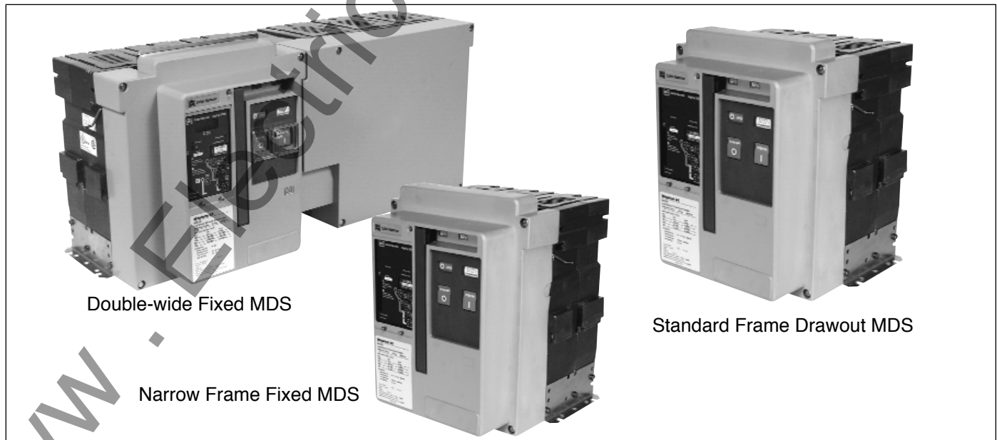
Figure 1-1 Family of Magnum DS (MDS) Low Voltage Power Fixed and Drawout Circuit Breakers (800-5000 Amperes)
