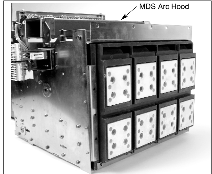
Figure 4-7 Typical MDS/MDSX Universal Cassette, 4-Pole (Flat Terminal Pads) (Shown with MDS Type Arc Hood)
