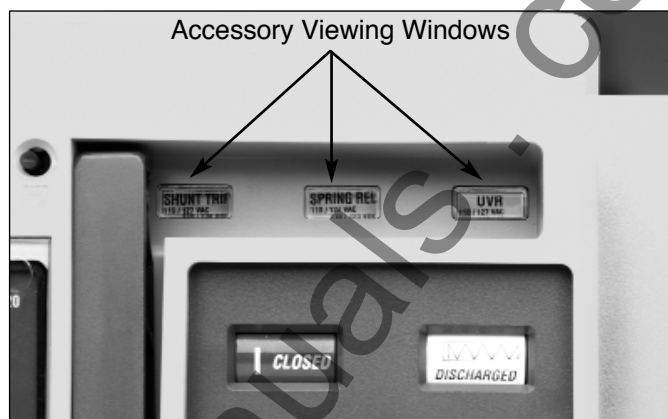
Figure 3-47 Through-the-Window Electrical Accessories
