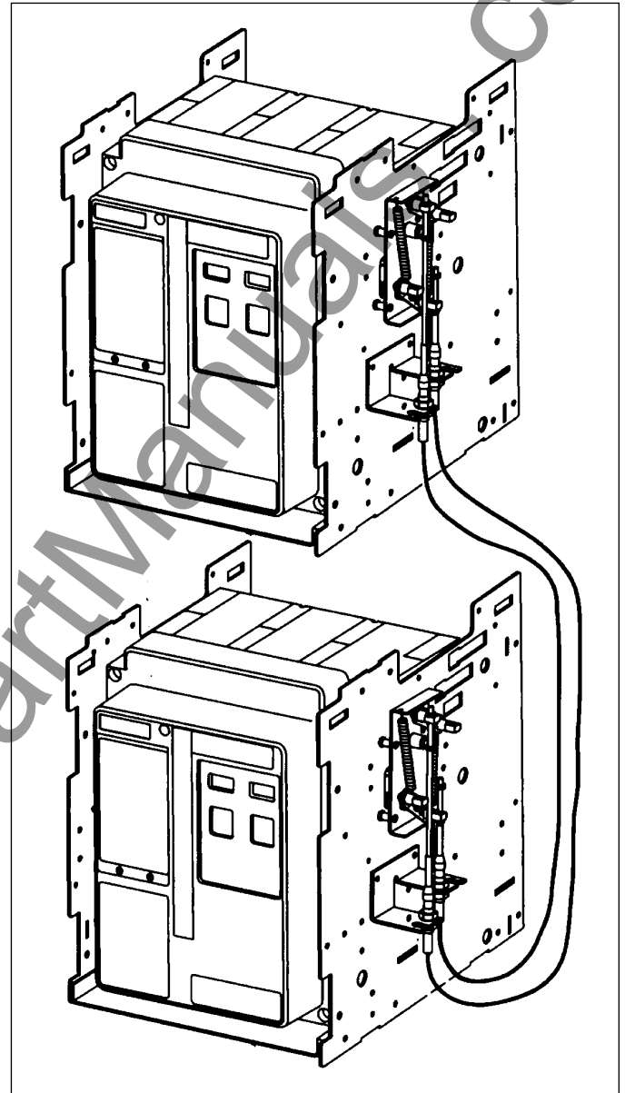
Figure 3-66 Cassette-Mounted 2-Way Cable Interlock
