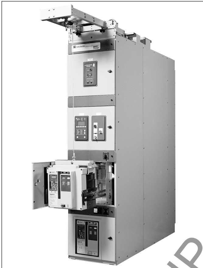
Figure 2-2 Magnum DS Circuit Breaker with Lifting Yoke Attached
