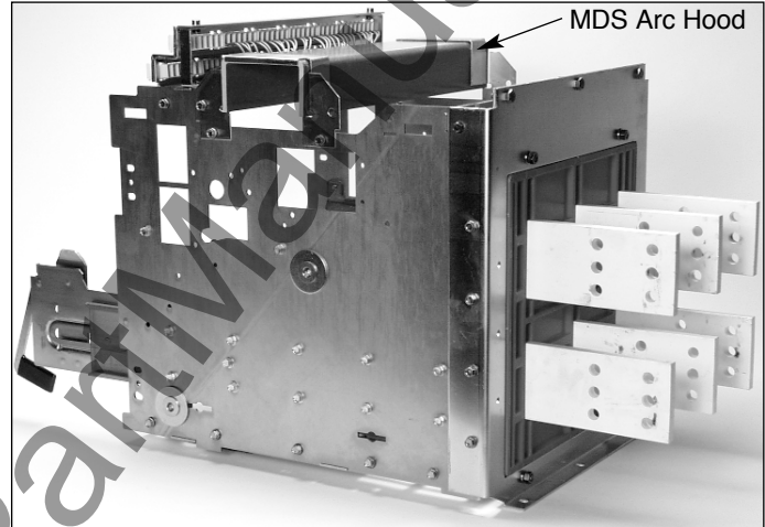
Figure 4-5 Typical MDS /MDSX Standard Cassette (Vertical Terminals) (Shown with MDS Type Arc Hood)
