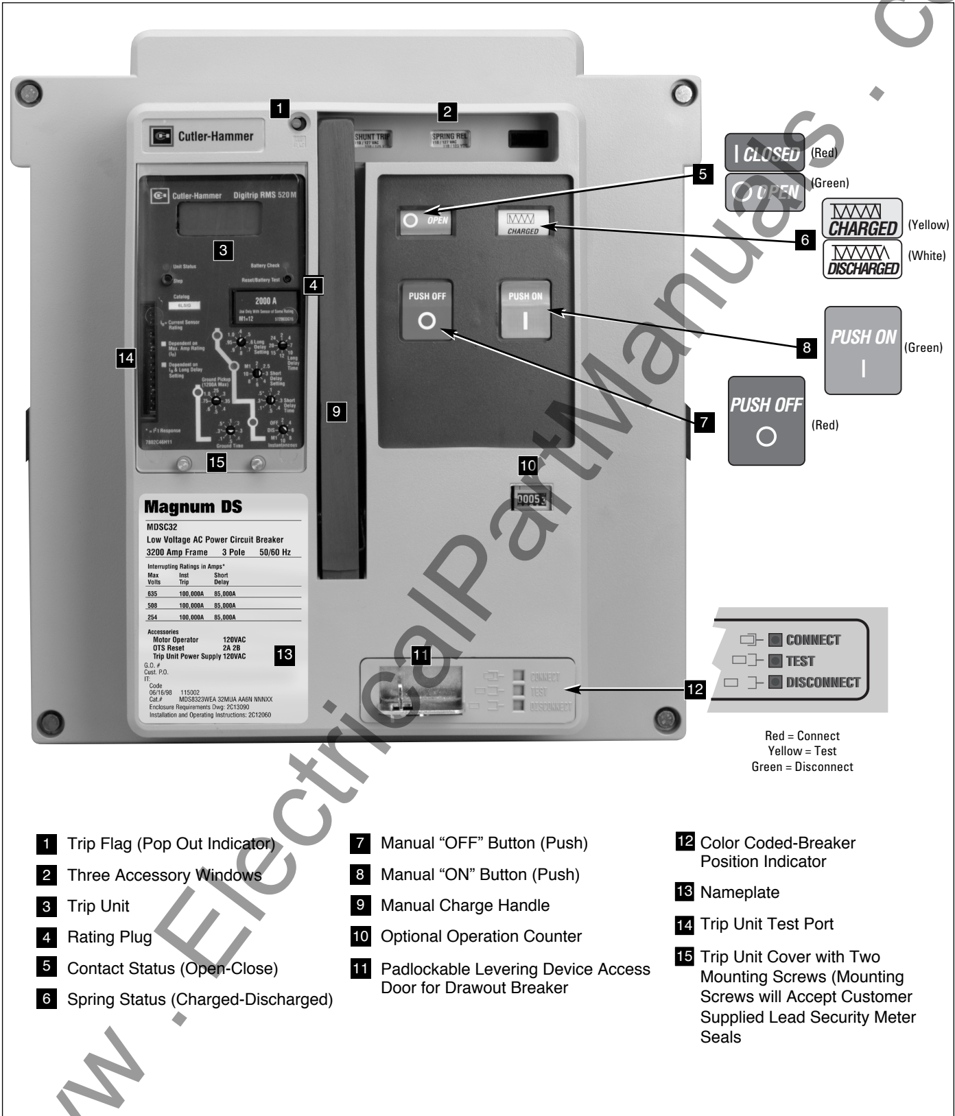
Figure 3-5 Typical Magnum DS/DSX Drawout Circuit Breaker Front Cover
