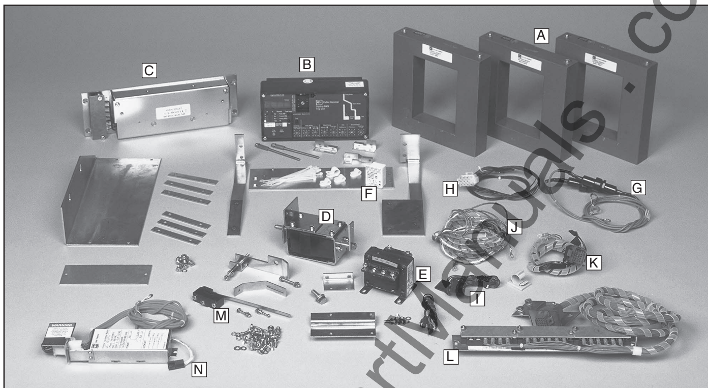
Fig. 39 Retrofit Components
