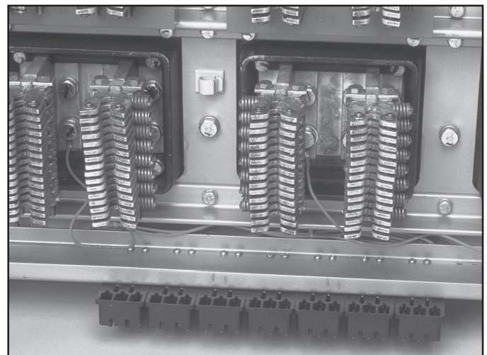
Fig. 21 PT Wires Connected to the Finger Clusters
