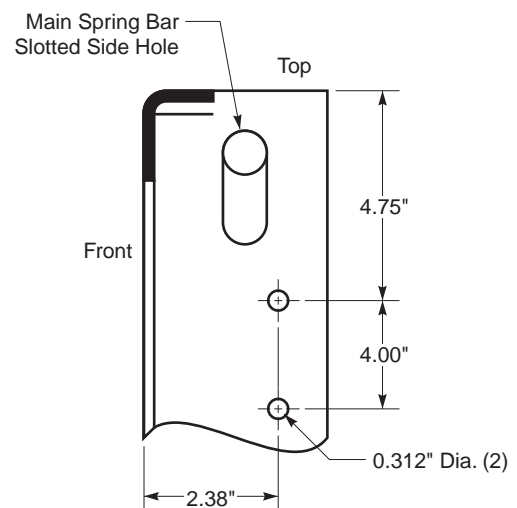
Drilling Plan "C"
