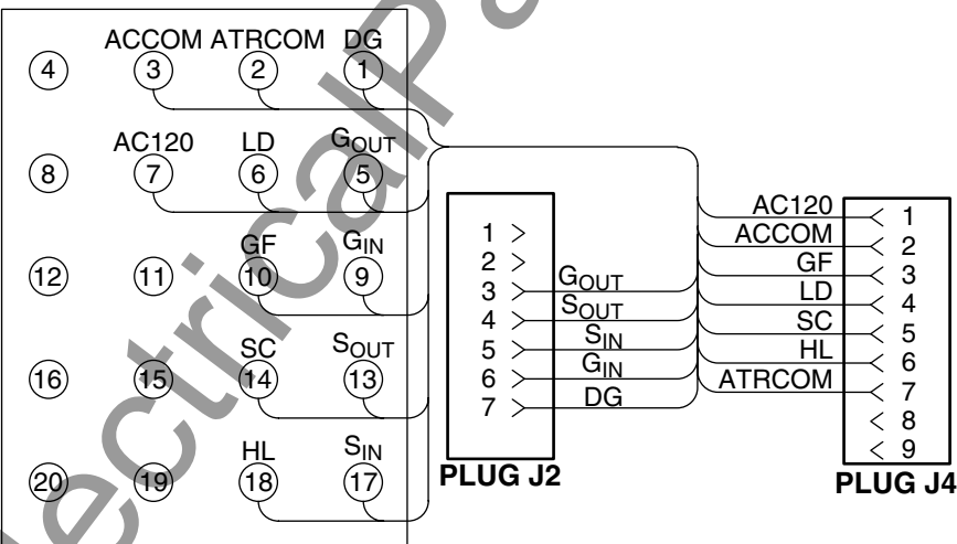
Fig. 12-9 Digitrip RMS 610 External Harness
