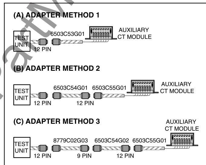
Fig. 8-2 Adapter Methods
