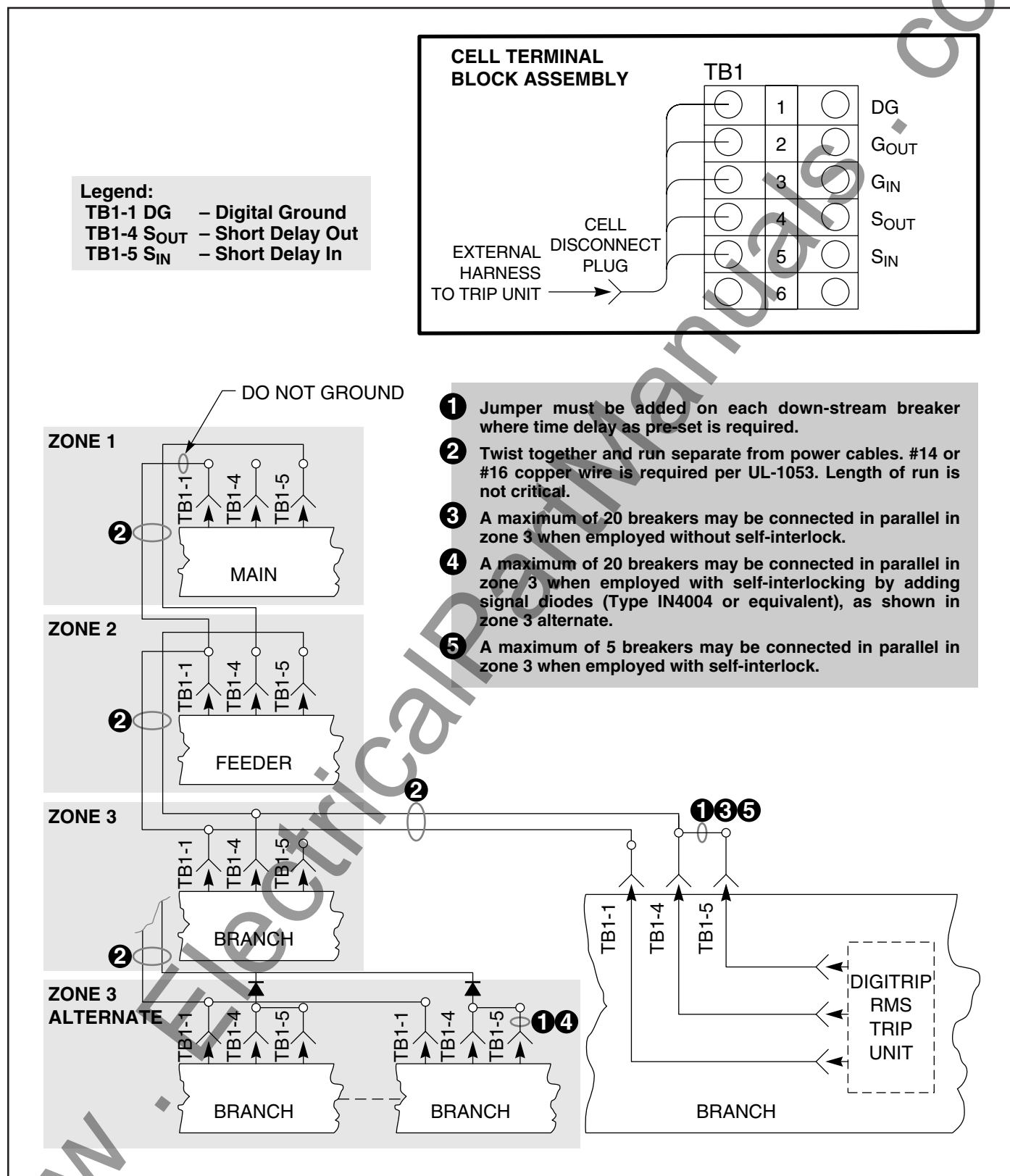
Fig. 10-3 Connection Schematics for Multiple Circuit Breakers
